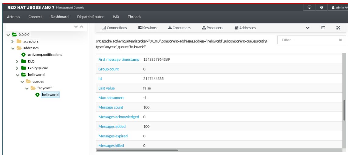
Figure 4.1. Message count
