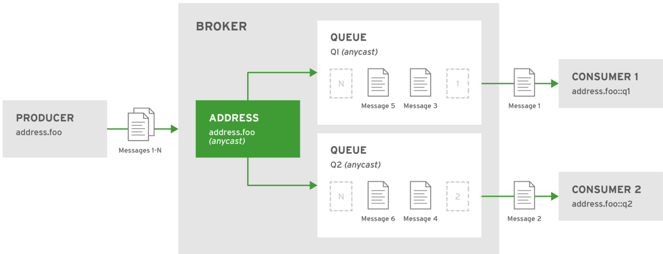
Figure 2.2. Point-to-point messaging with two queues
