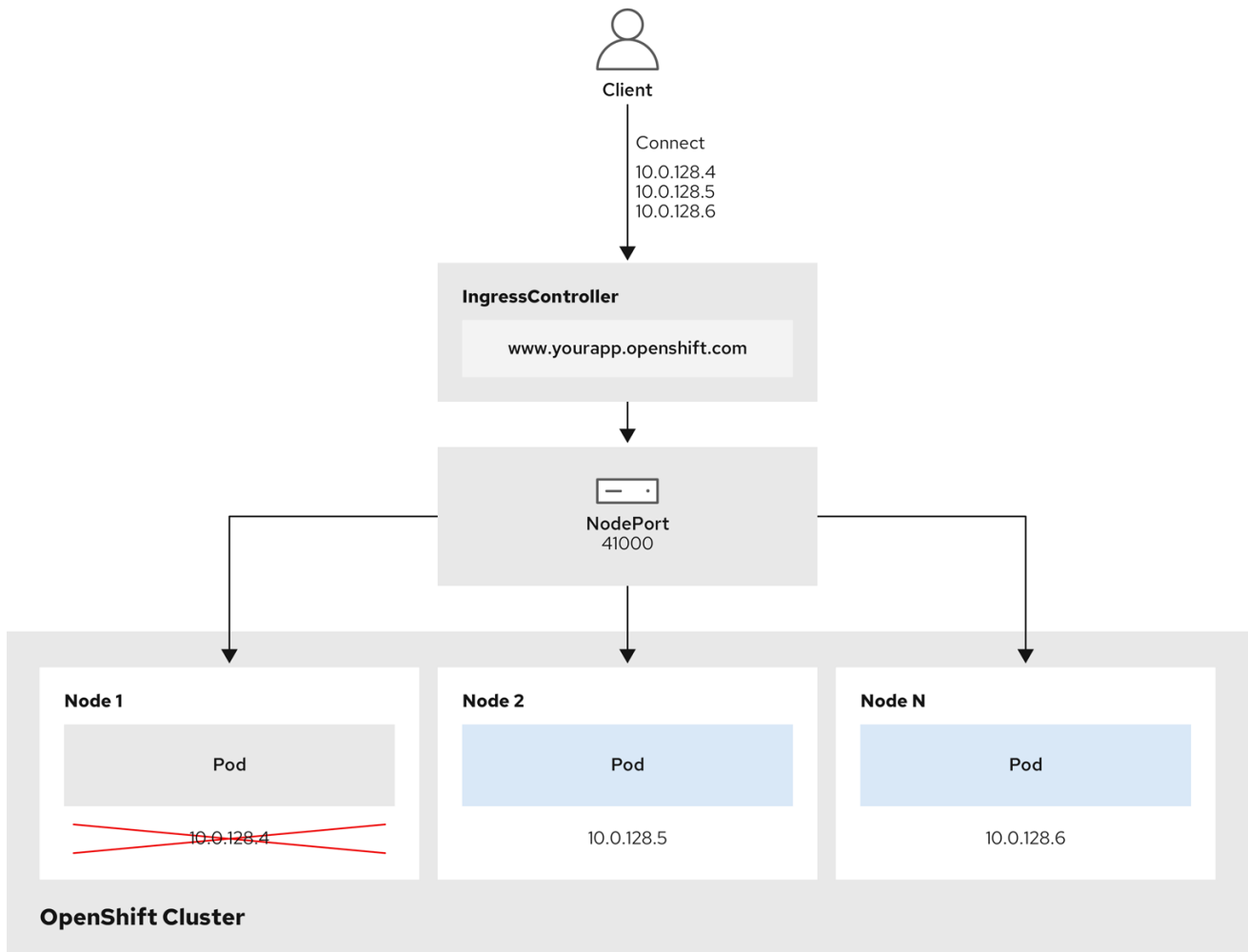
Figure 6.1. Diagram of NodePortService
