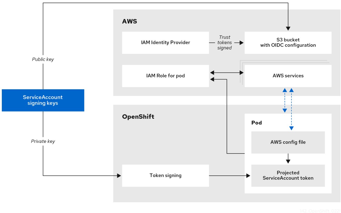
Figure 18.1. STS authentication flow
