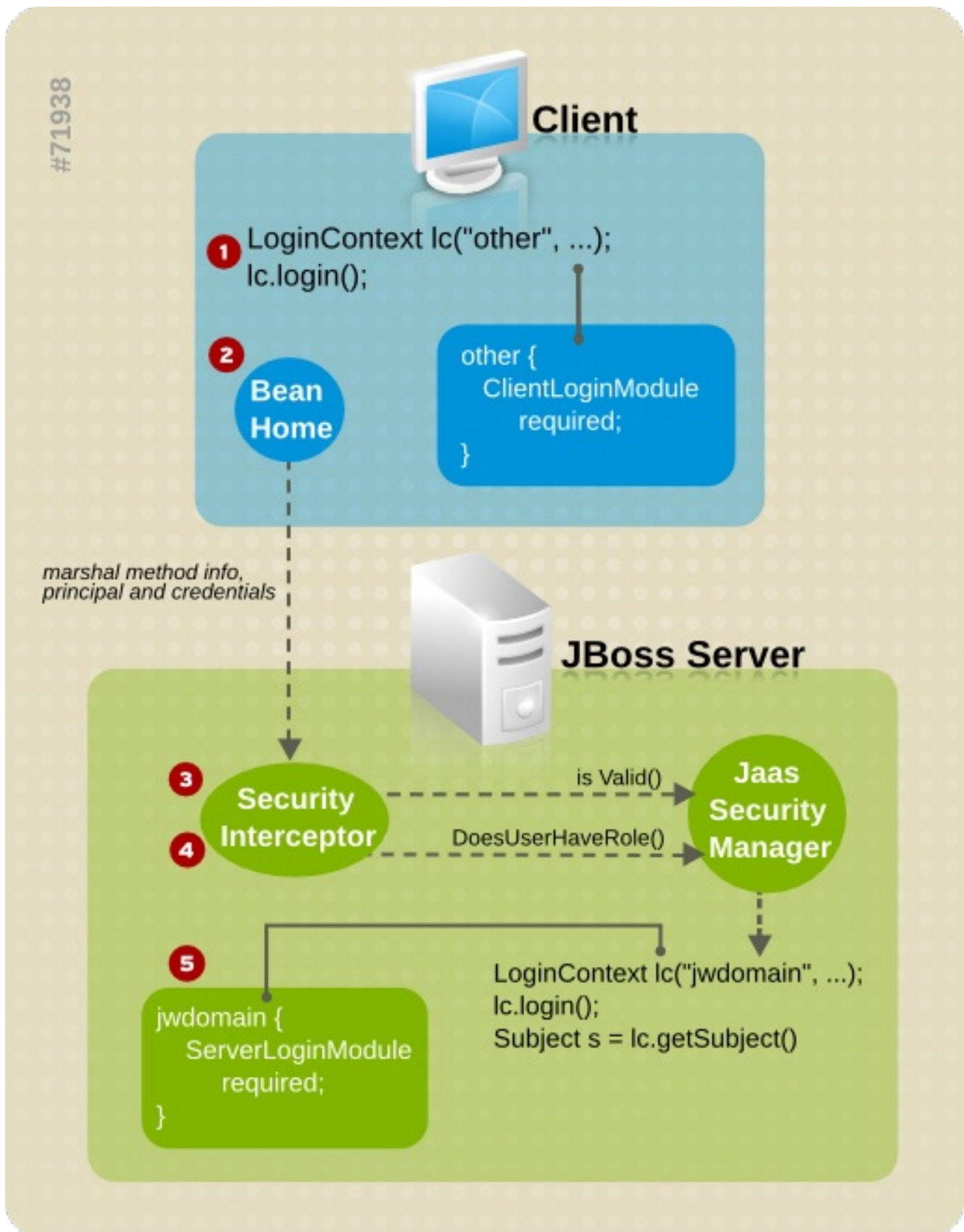
Figure 13.1. Steps of a Secured EJB Method Invocation
