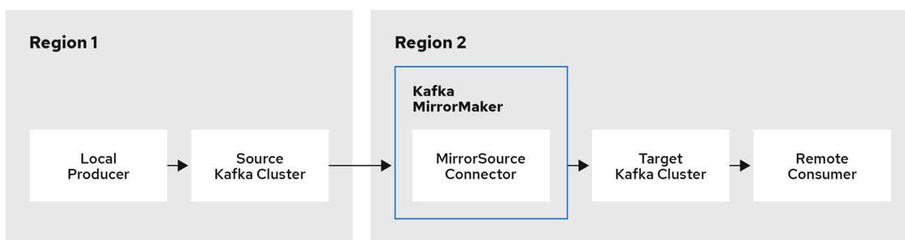
Figure 8.1. Replication across two clusters
