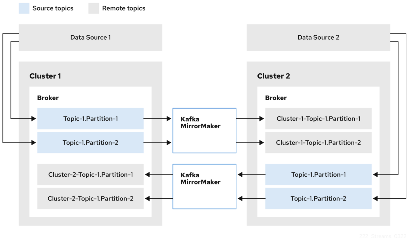
Figure 8.2. Topic renaming
