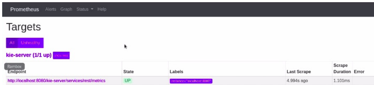
Figure 17.2. Prometheus expression browser with Process Server target
