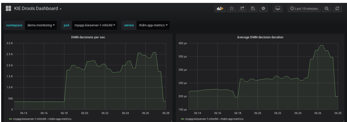
Figure 17.8. Grafana dashboard with Process Server metrics for DMN models
