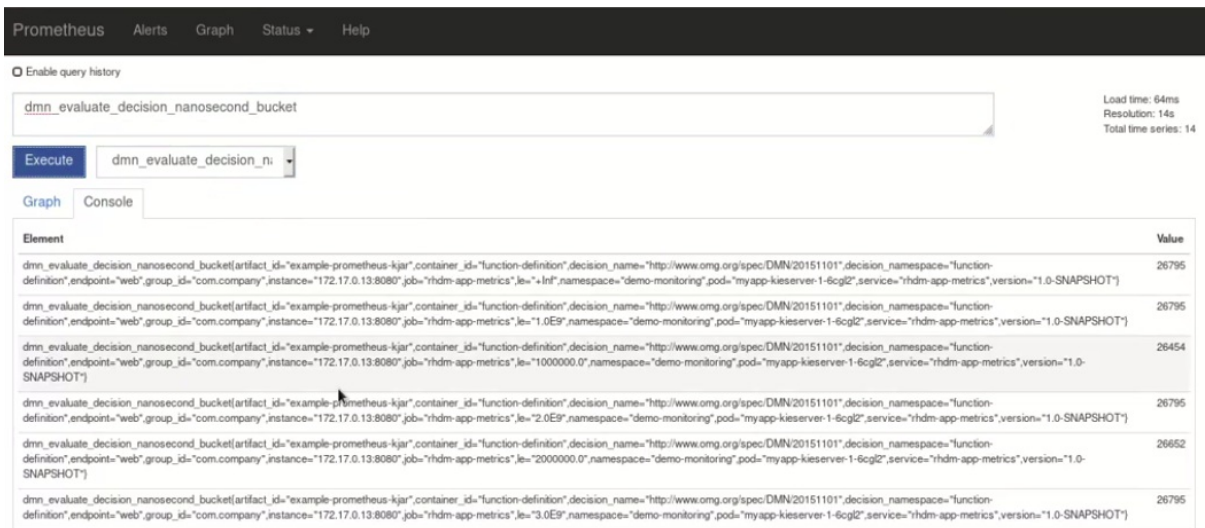
Figure 17.6. Prometheus expression browser with Process Server metrics
