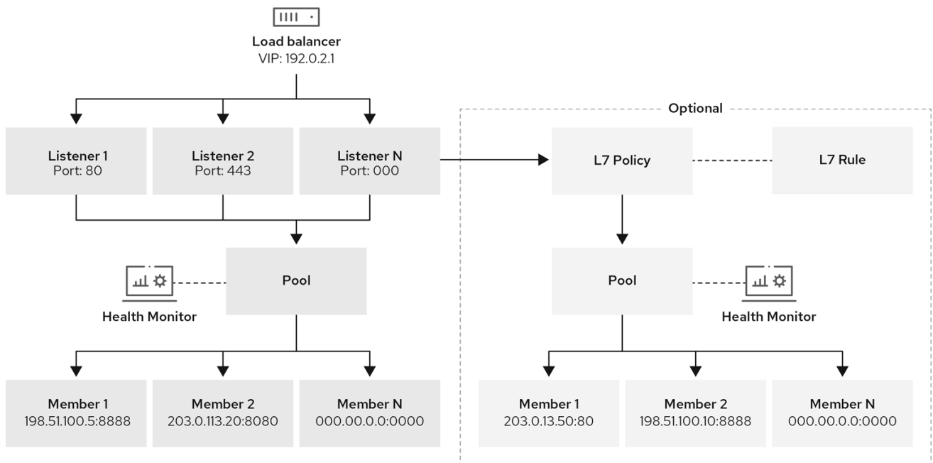
Figure 1.2. Load-balancing service object model diagram
