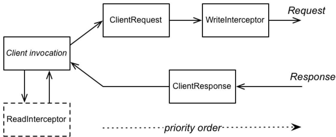
Figure 59.2. Client-Side Filter and Interceptor Extension Points
