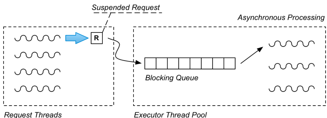
Figure 47.1. Threading Model for Asynchronous Processing
