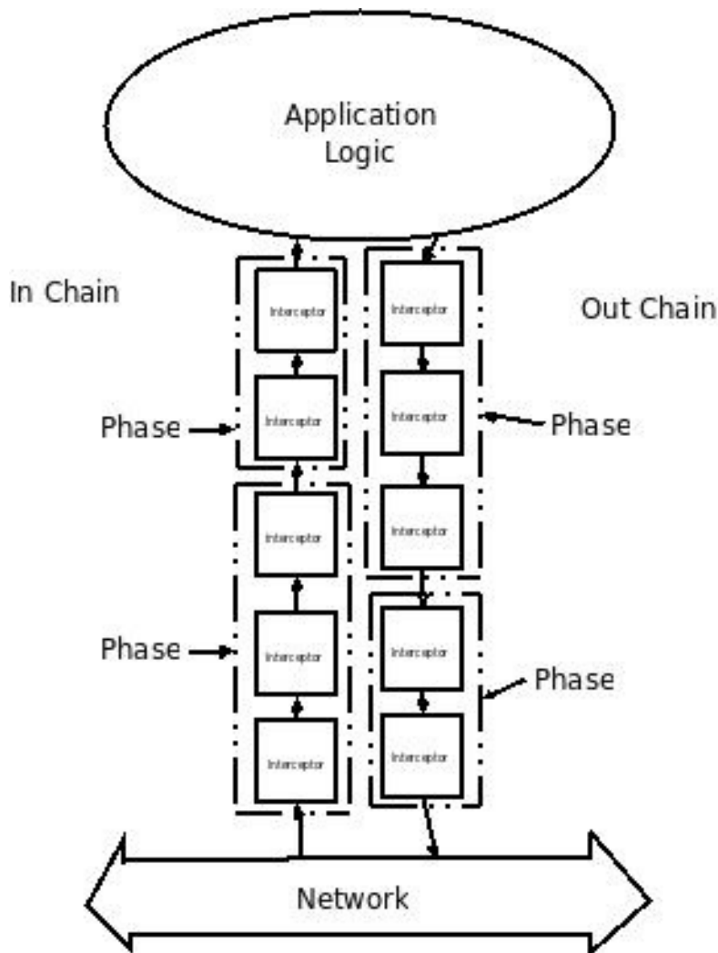
Figure 53.1. Apache CXF interceptor chains
