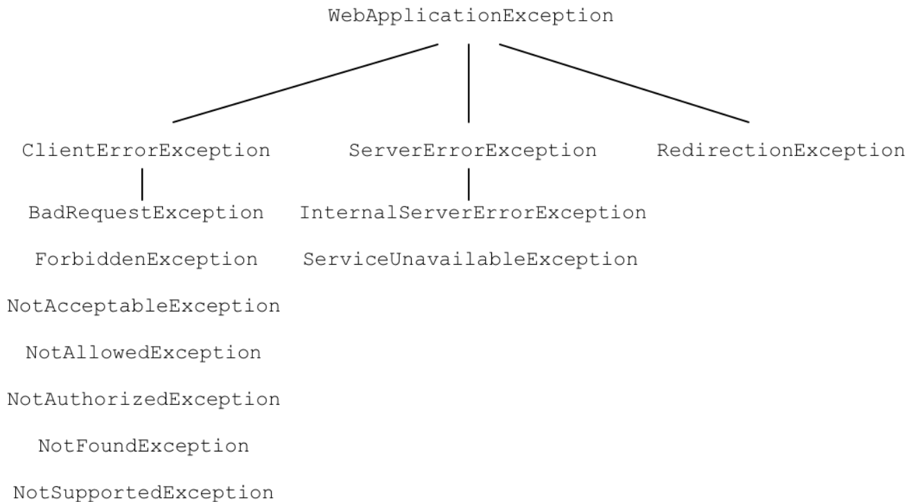
Figure 48.1. JAX-RS 2.0 Application Exception Hierarchy
