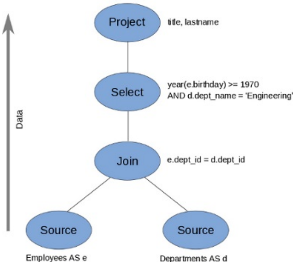
Figure 13.1. Canonical Query Plan
