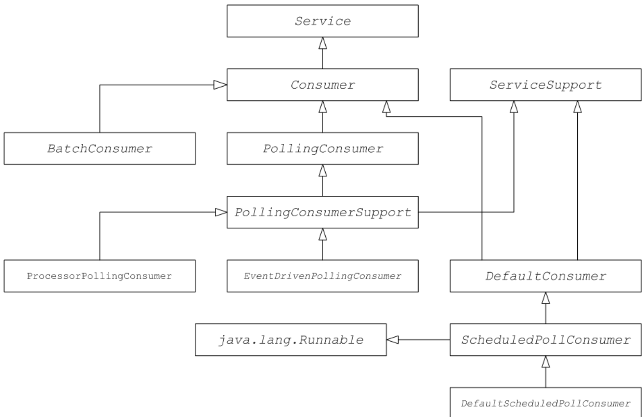
Figure 40.1. Consumer Inheritance Hierarchy
