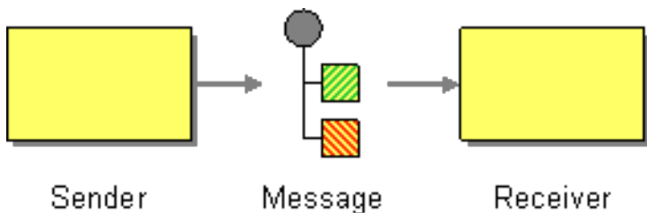
Figure 5.1. Message Pattern
