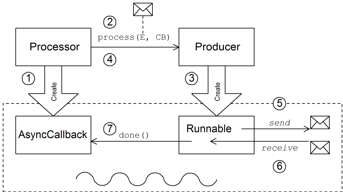
Figure 37.7. Asynchronous Producer
