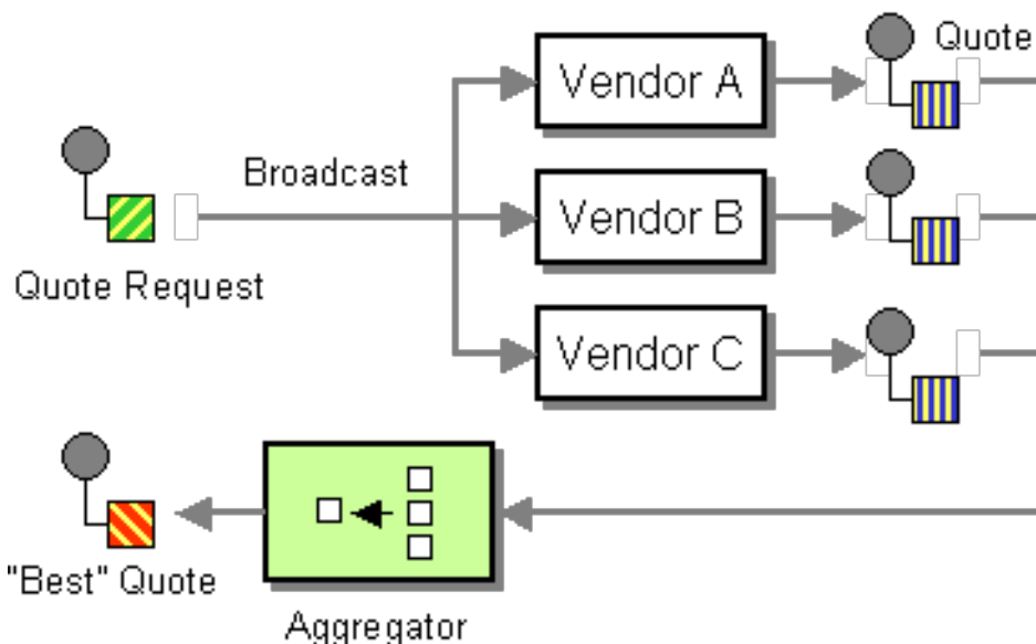
Figure 8.12. Scatter-Gather Pattern
