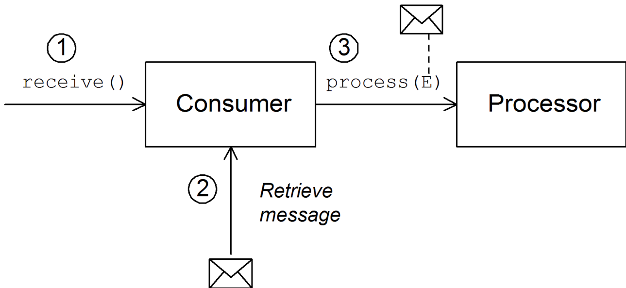
Figure 37.5. Polling Consumer
