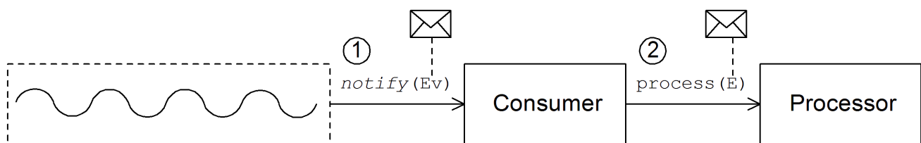
Figure 37.3. Event-Driven Consumer
