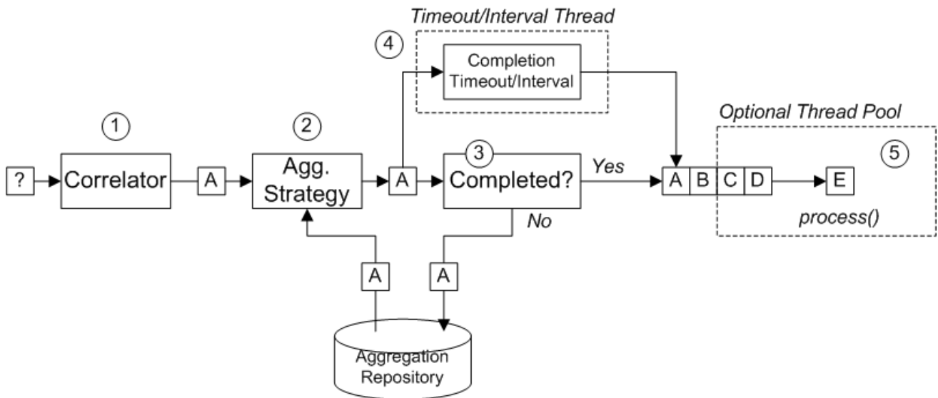
Figure 8.6. Aggregator Implementation
