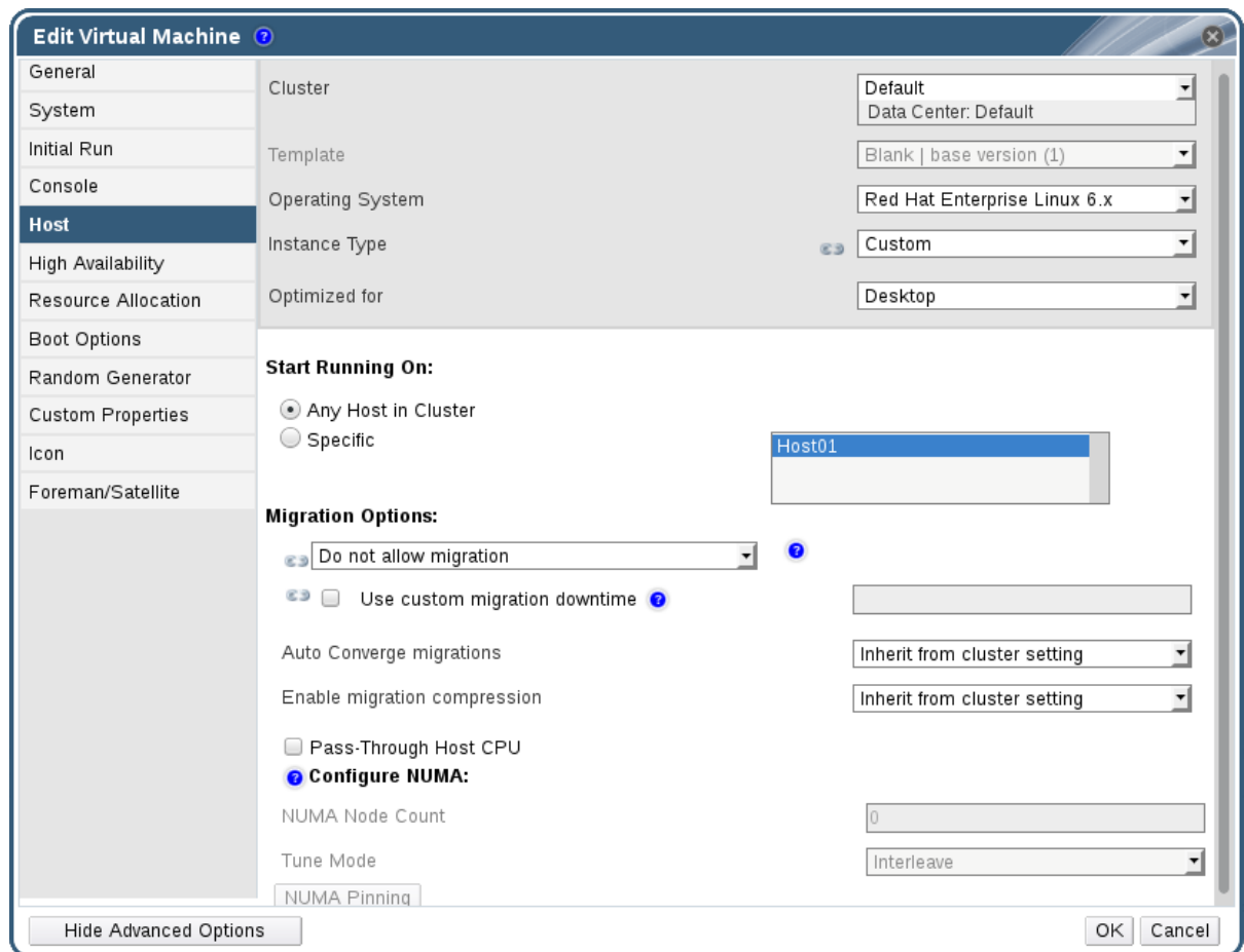
Figure 6.15. The Edit Virtual Machine Window
