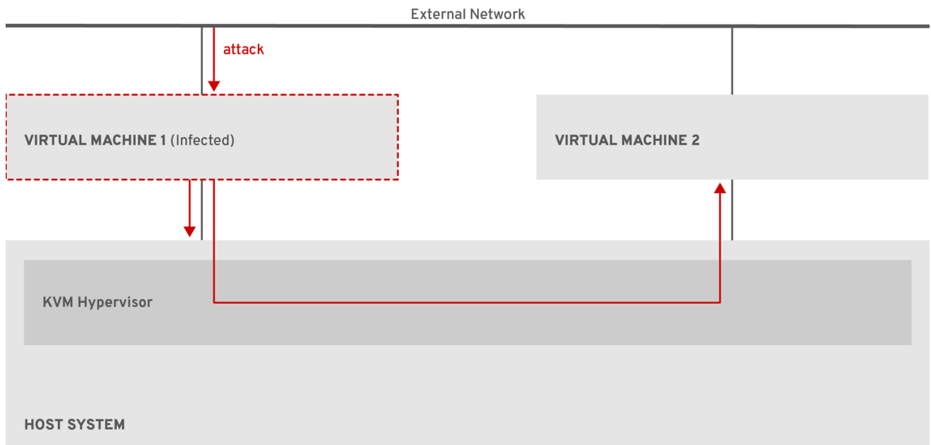
Figure 18.1. A potential malware attack vector on a virtualization host
