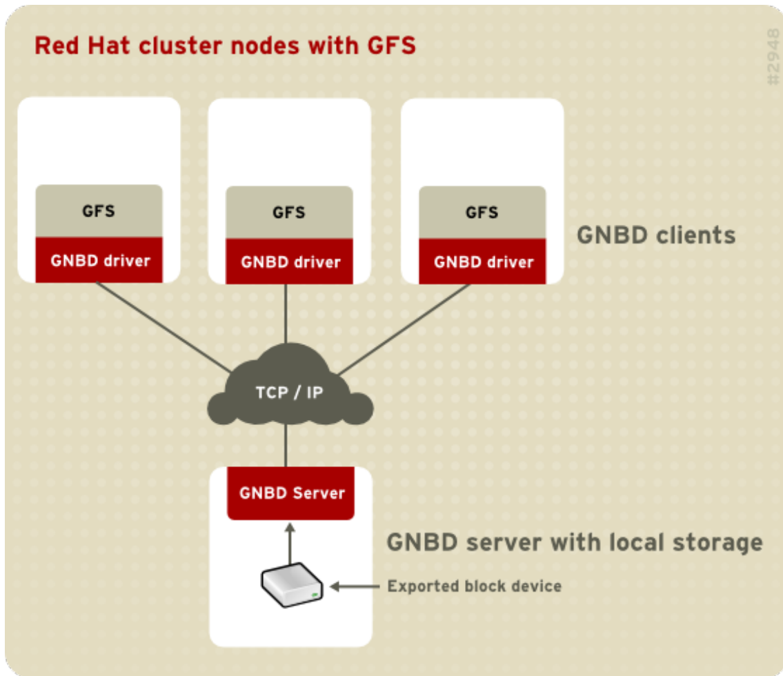
Figure 1.19. GNBD Overview
