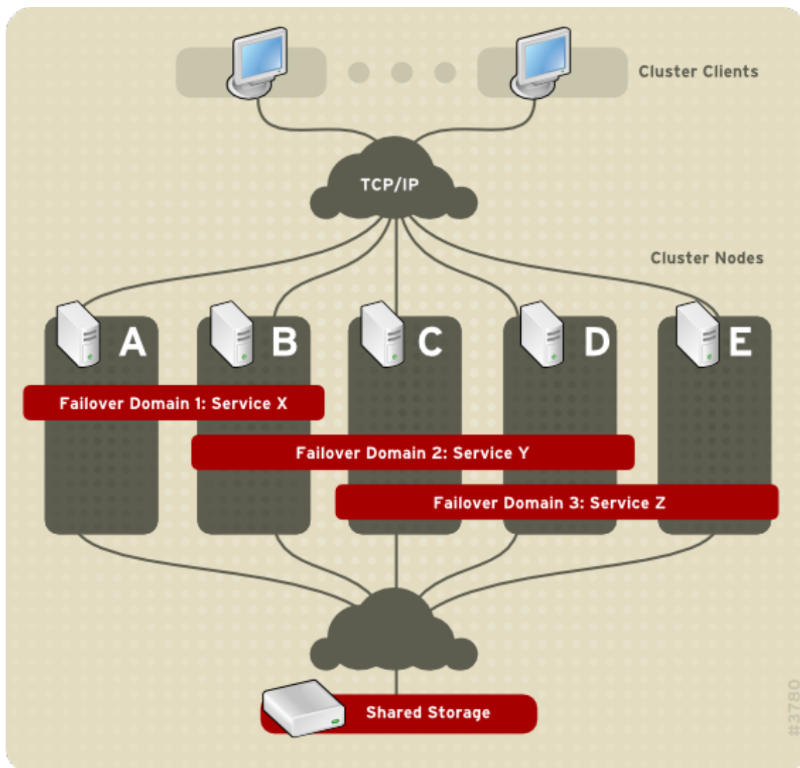
Figure 1.10. Failover Domains
