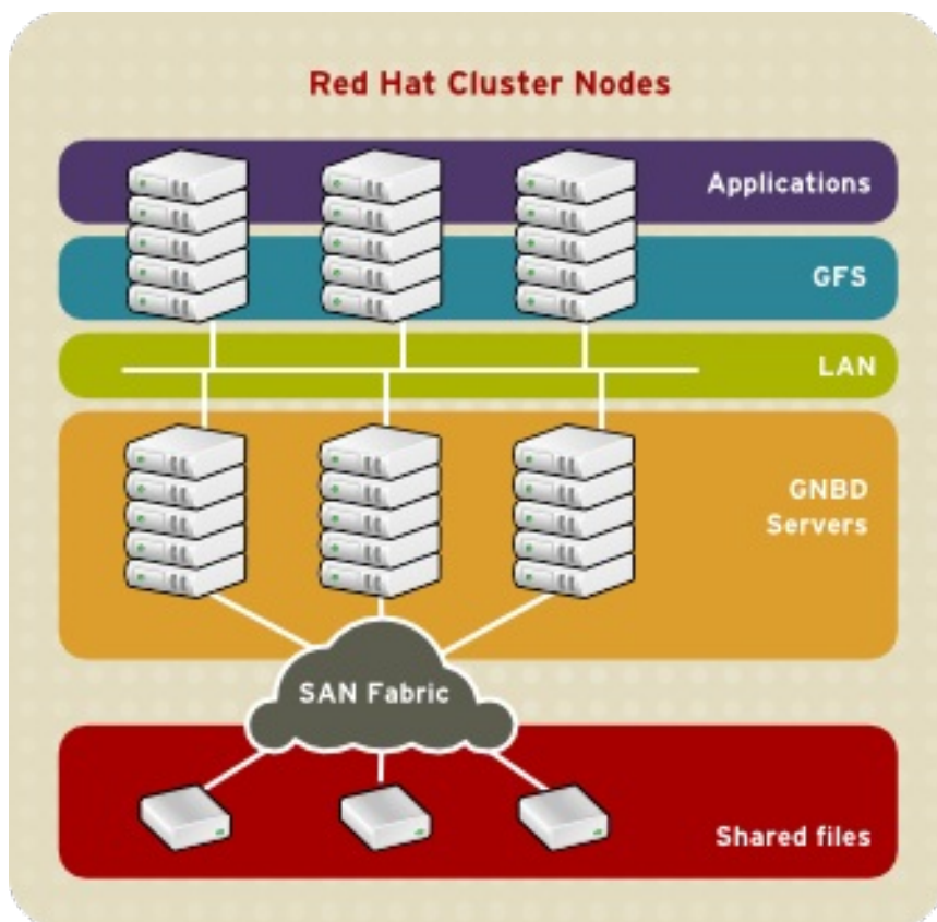
Figure 1.13. GFS and GNBD with a SAN
