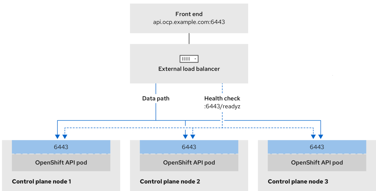
Figure 23.5. Example network workflow that shows an OpenShift API operating in an OpenShift Container Platform environment
