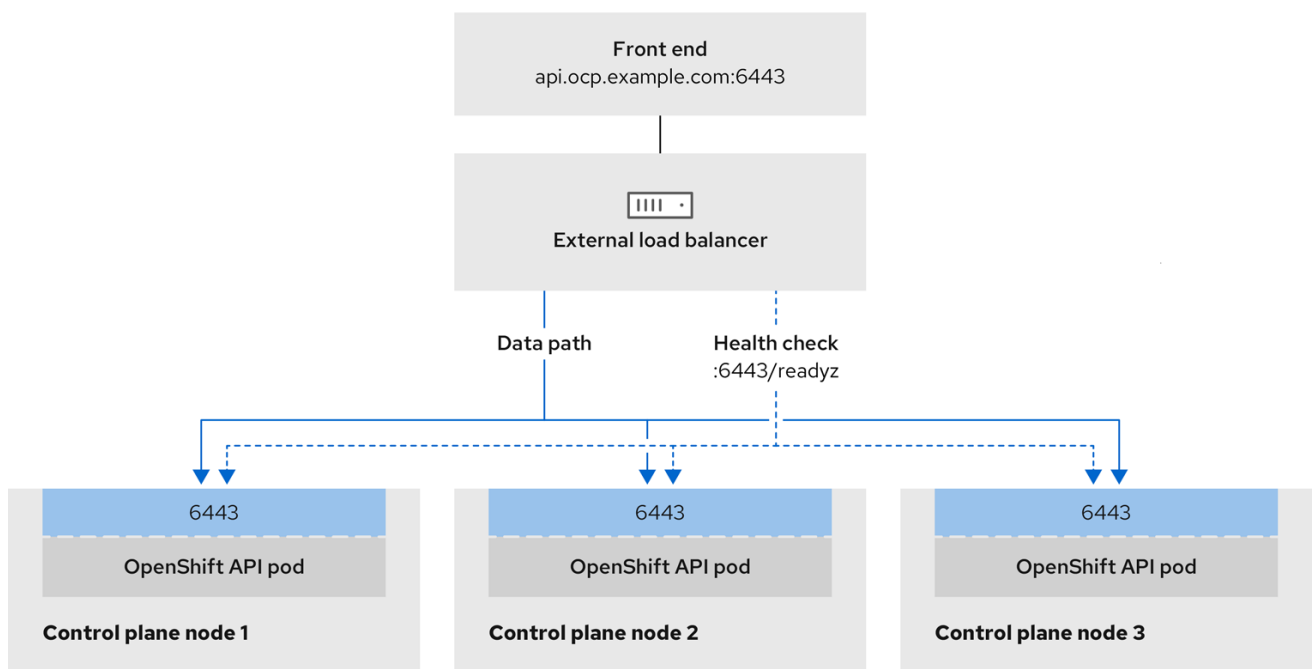
Figure 16.2. Example network workflow that shows an OpenShift API operating in an OpenShift Container Platform environment
