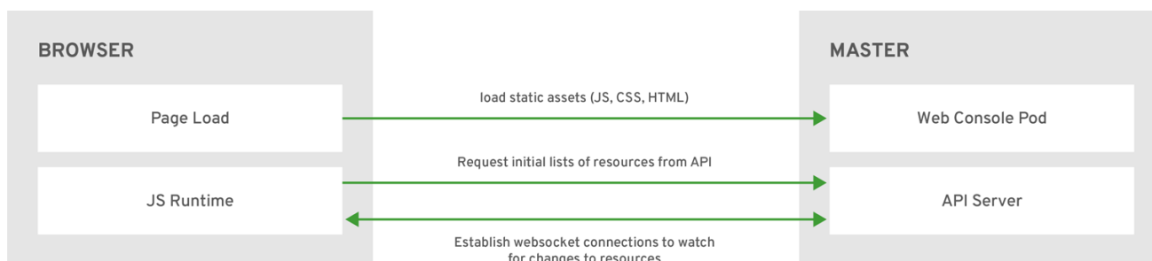
Figure 2.3. Web Console Request Architecture
