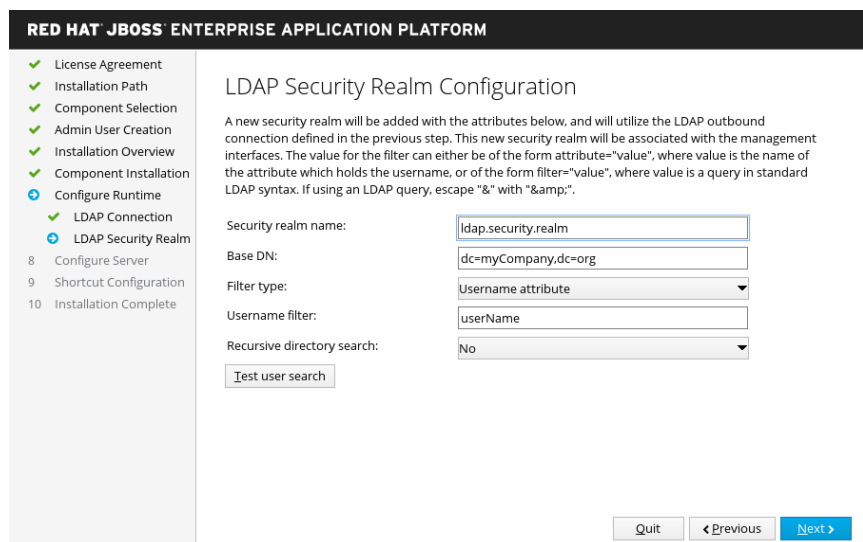
Figure 3.5. JBoss EAP Installer - LDAP Security Realm Configuration Screen
