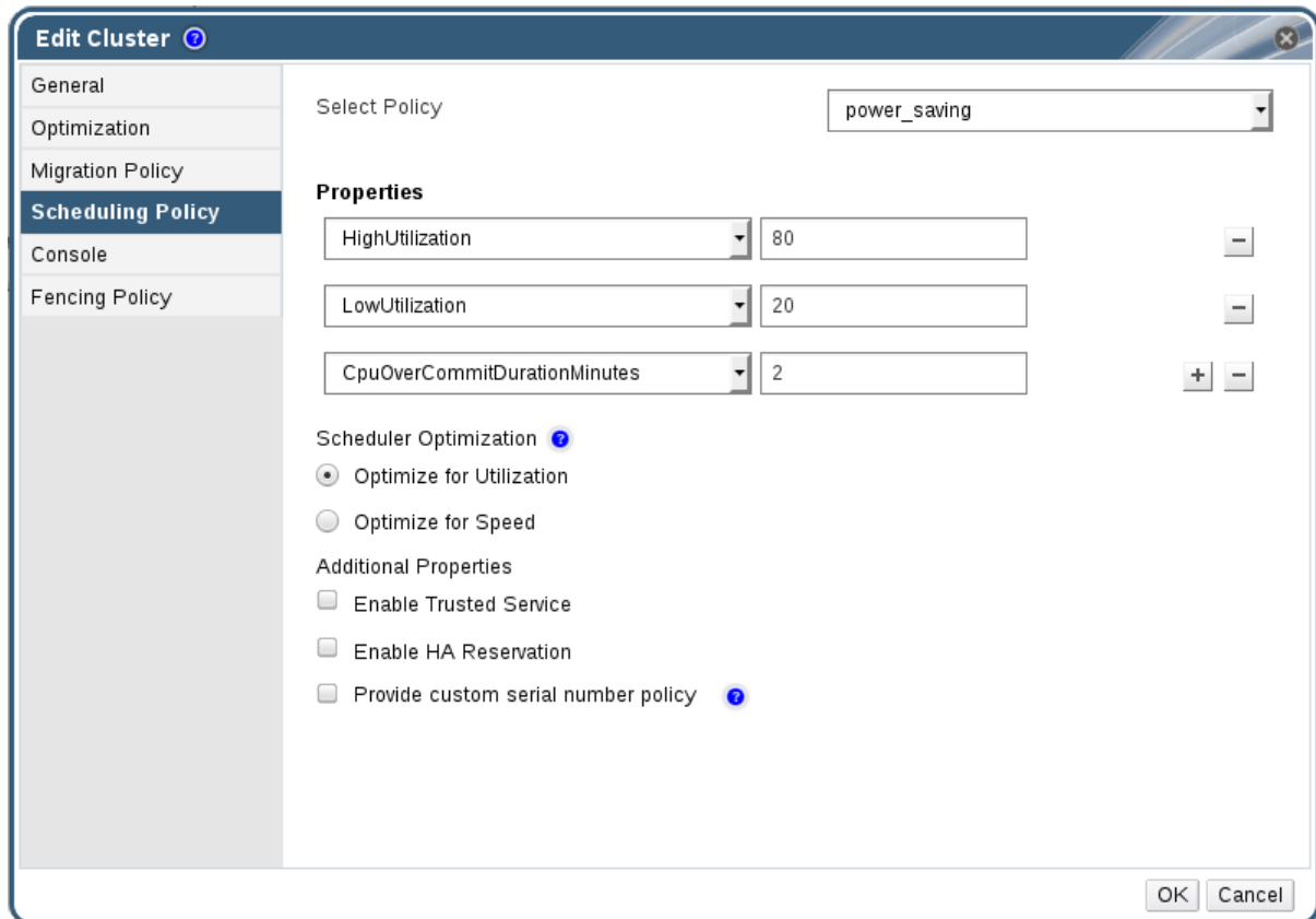
Figure 5.4. Edit Scheduling Policy
