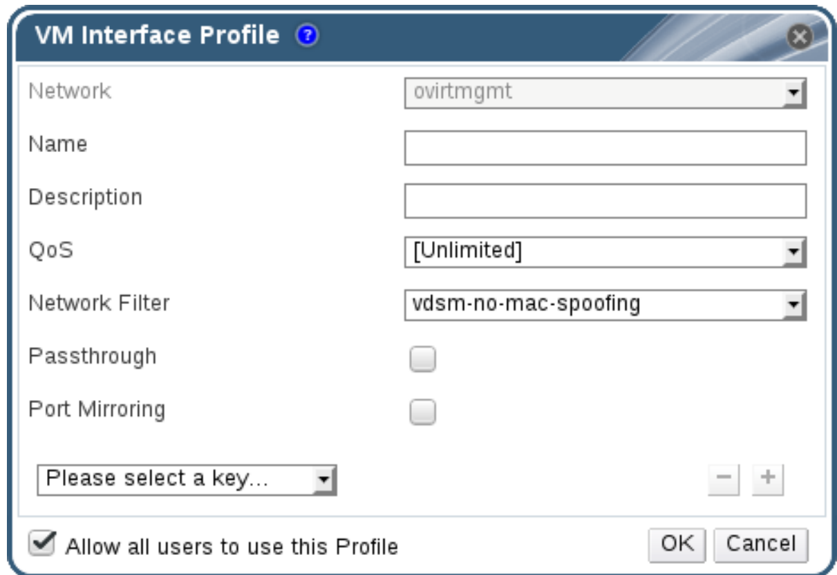
Figure 6.2. The VM Interface Profile window
