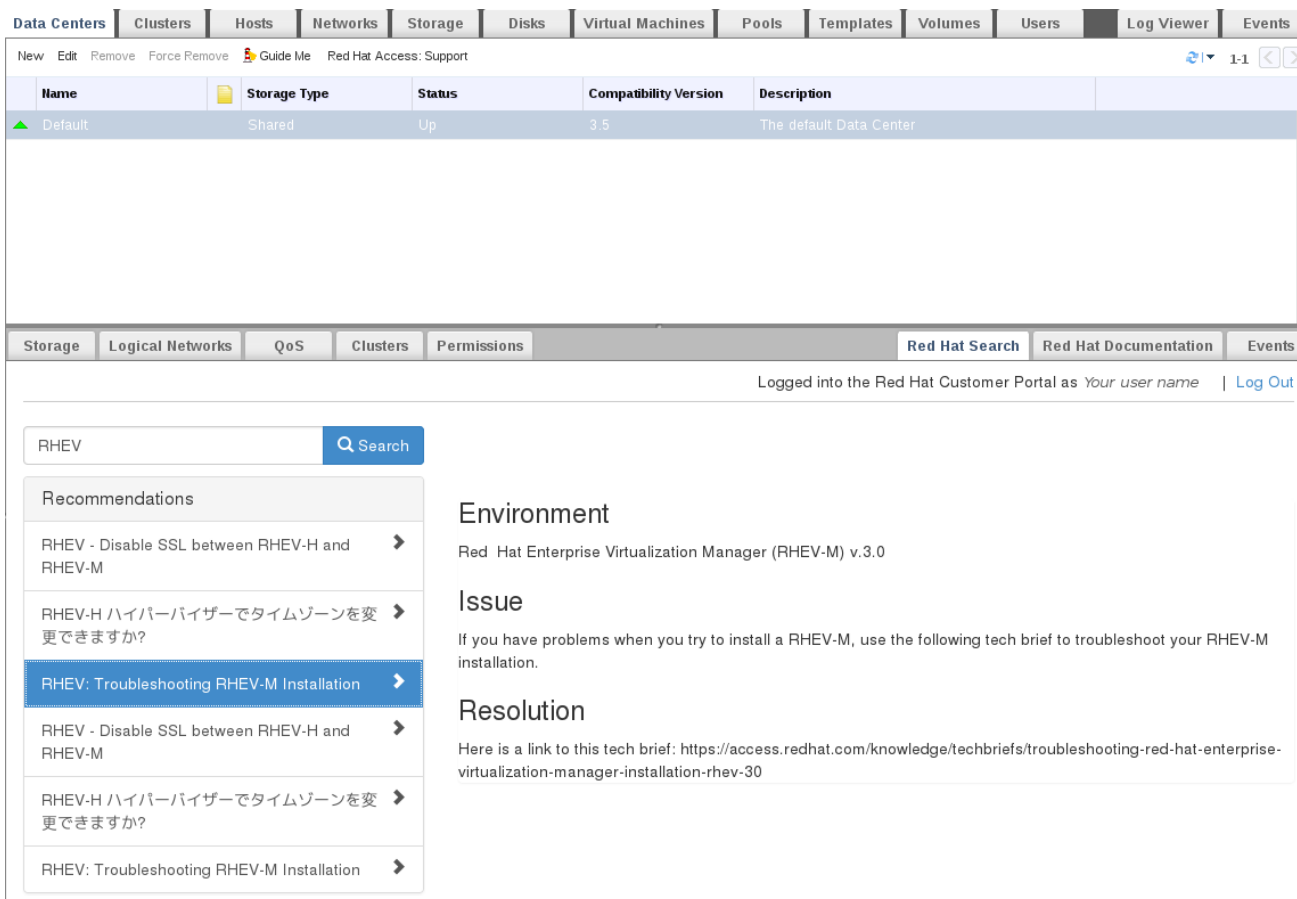
Figure C.3. Red Hat Support Plug-in - Query Results in the Left-Hand Navigation List
