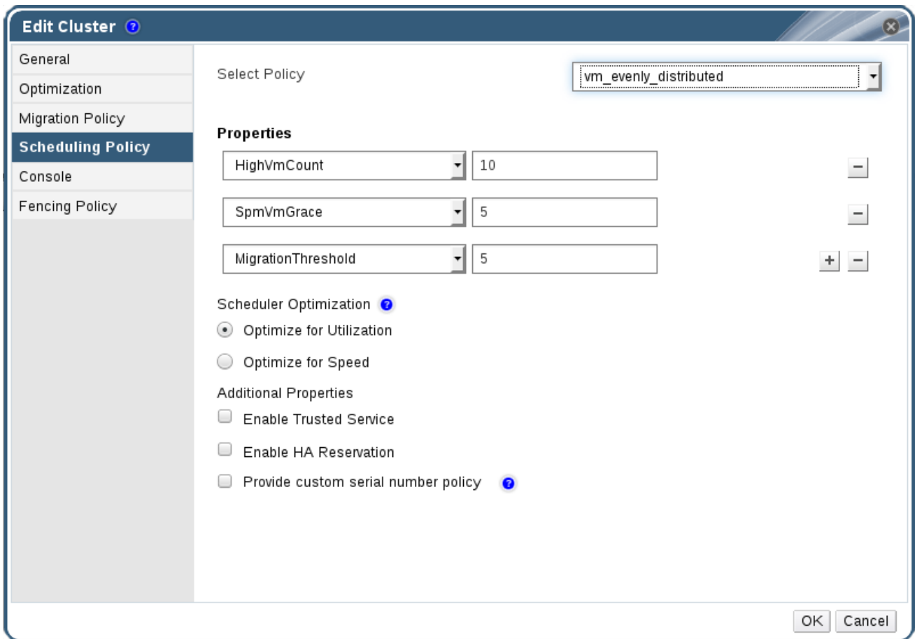
Figure 5.3. Scheduling Policy Settings: vm_evenly_distributed
