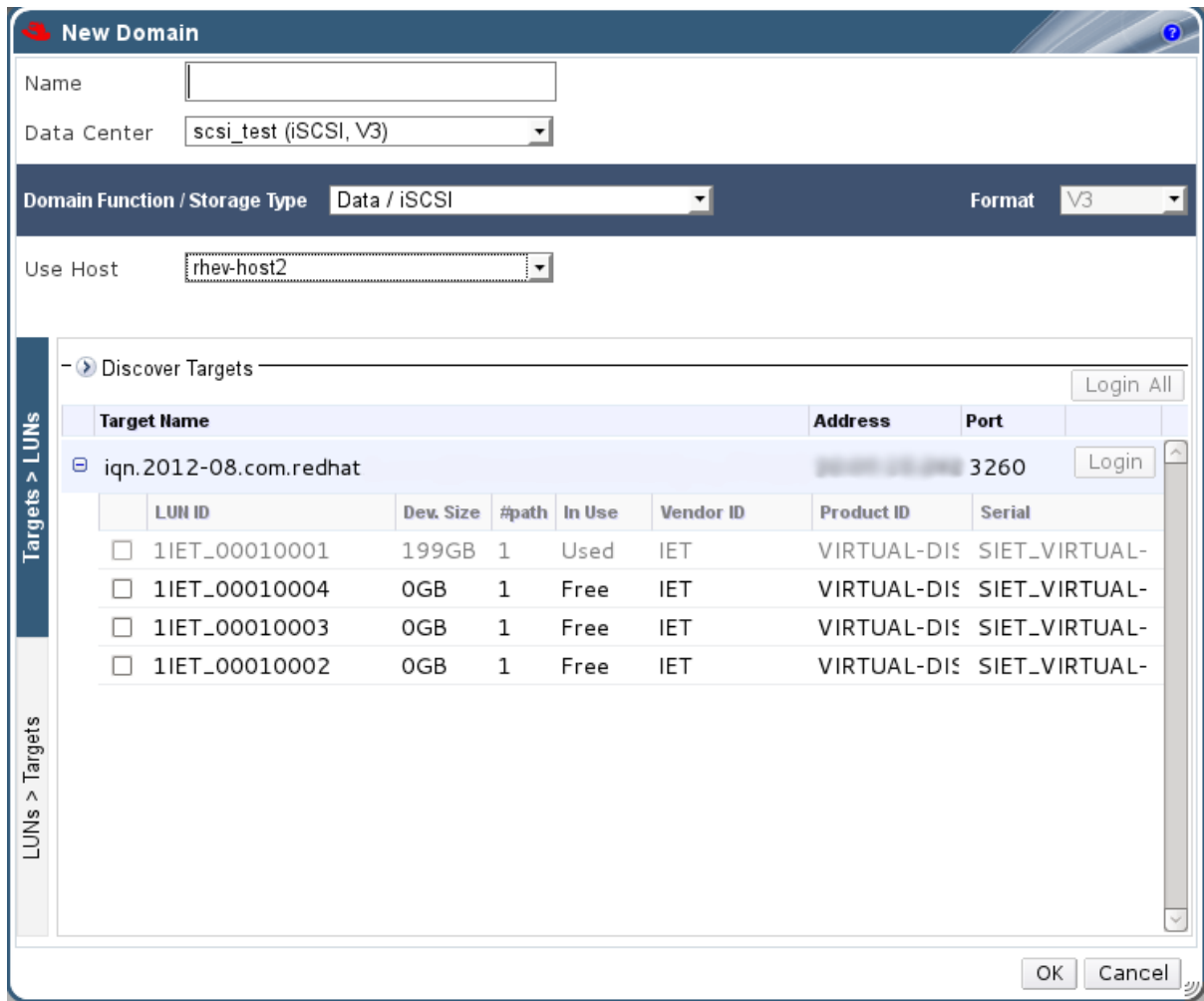
Figure 8.6. Unusable LUNs in the Red Hat Virtualization Administration Portal
