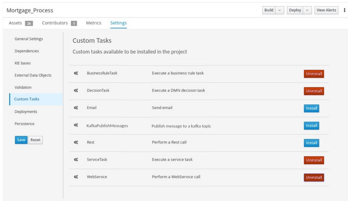
Figure 29.4. Install custom tasks for use in processes
