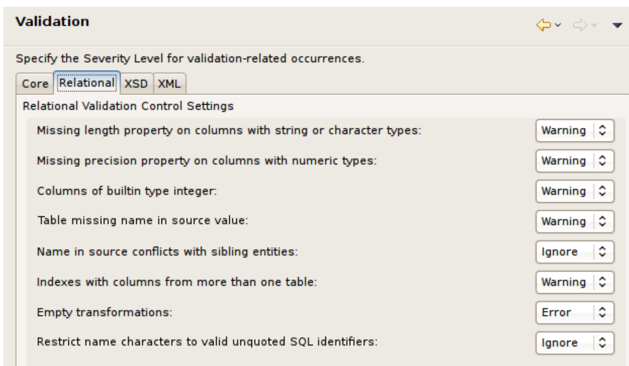
Figure B.10. Relational Model Validation Preferences Panel
