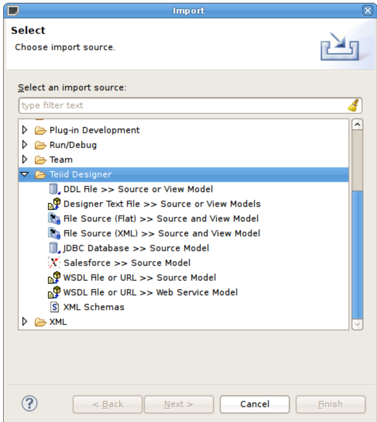
Figure 9.10. Import from Flat File Source
