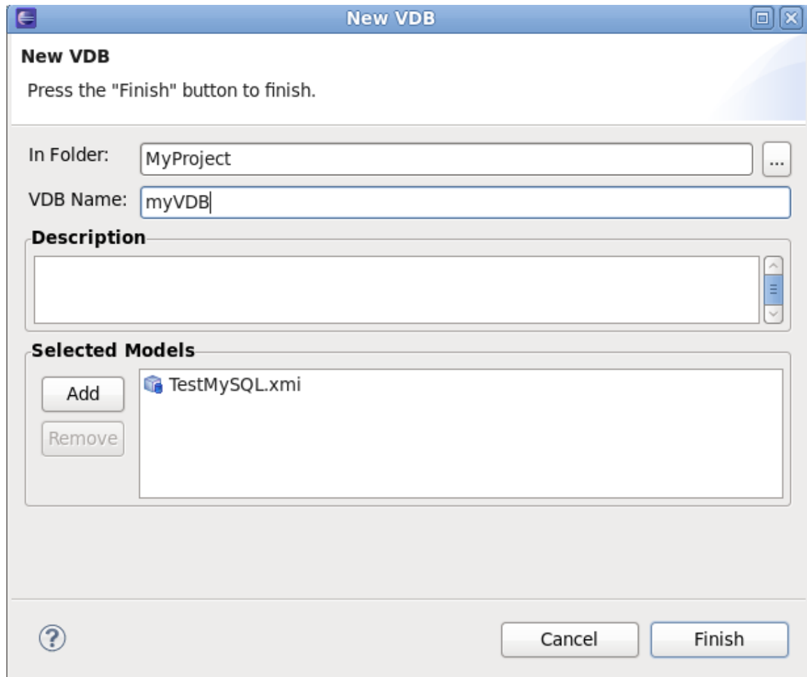
Figure 7.14. New VDB
