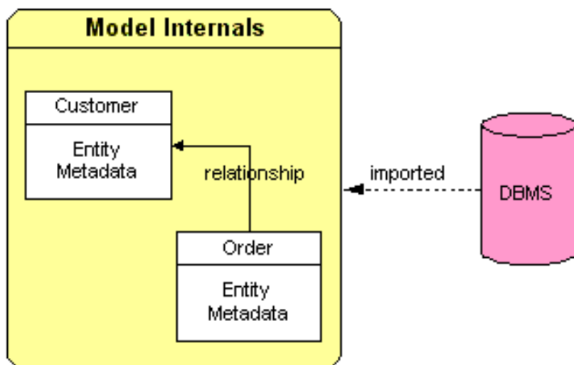
Figure 2.2. Model Internals
