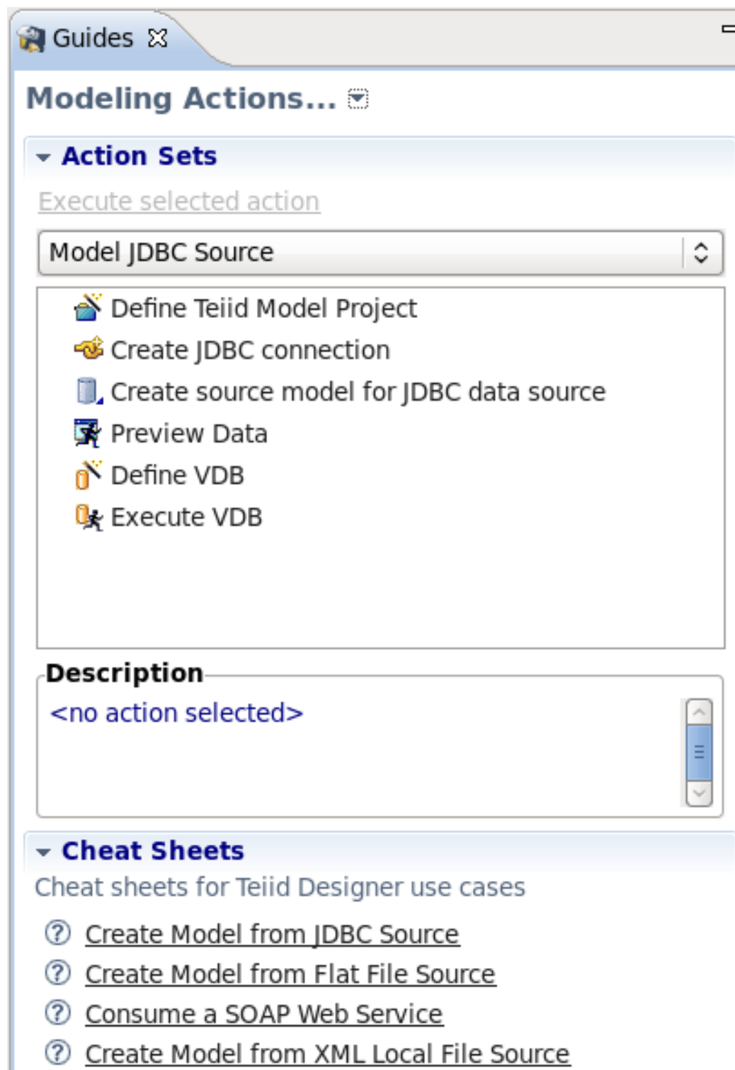
Figure 7.1. Guides View
