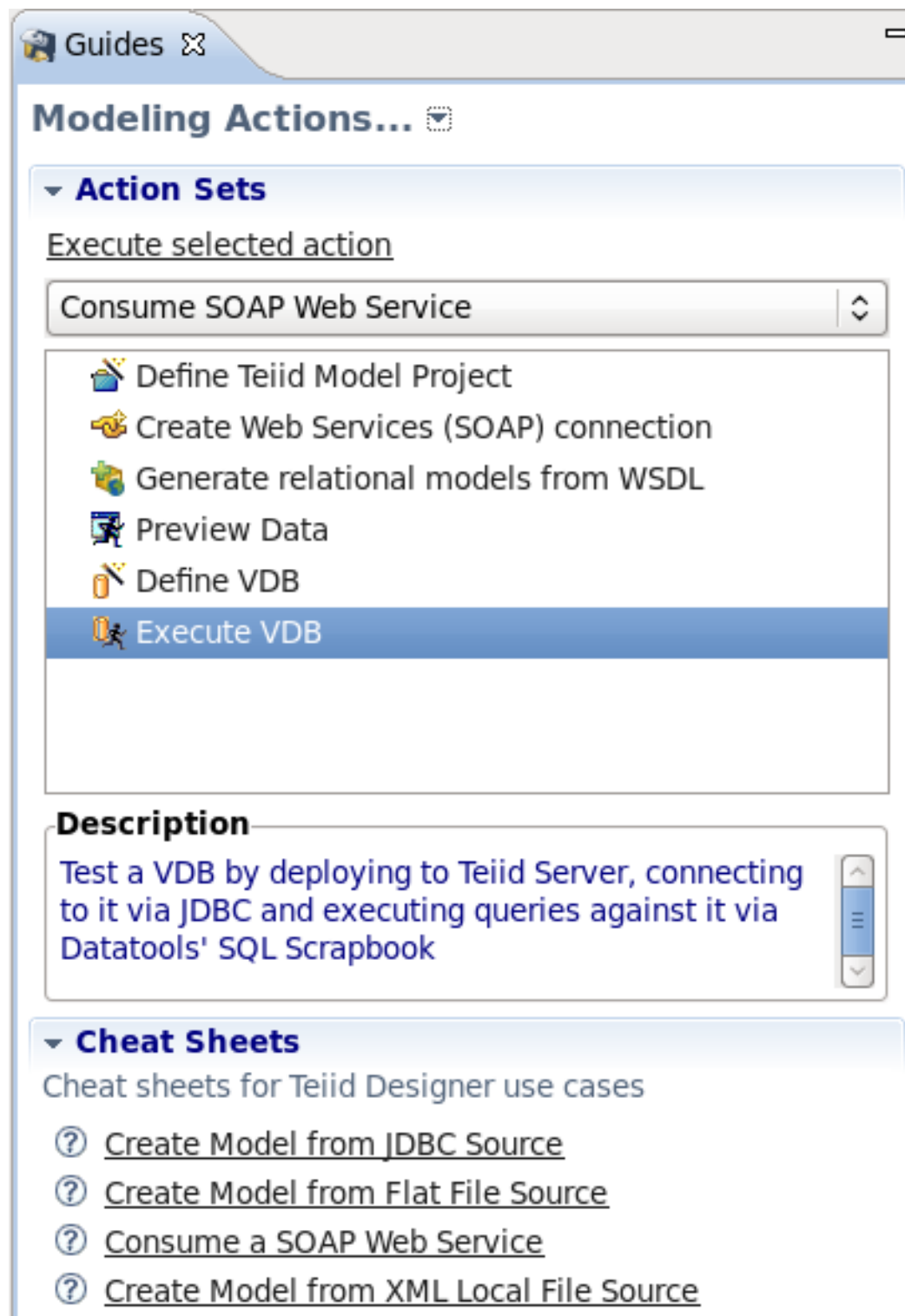
Figure 7.17. Guides View
