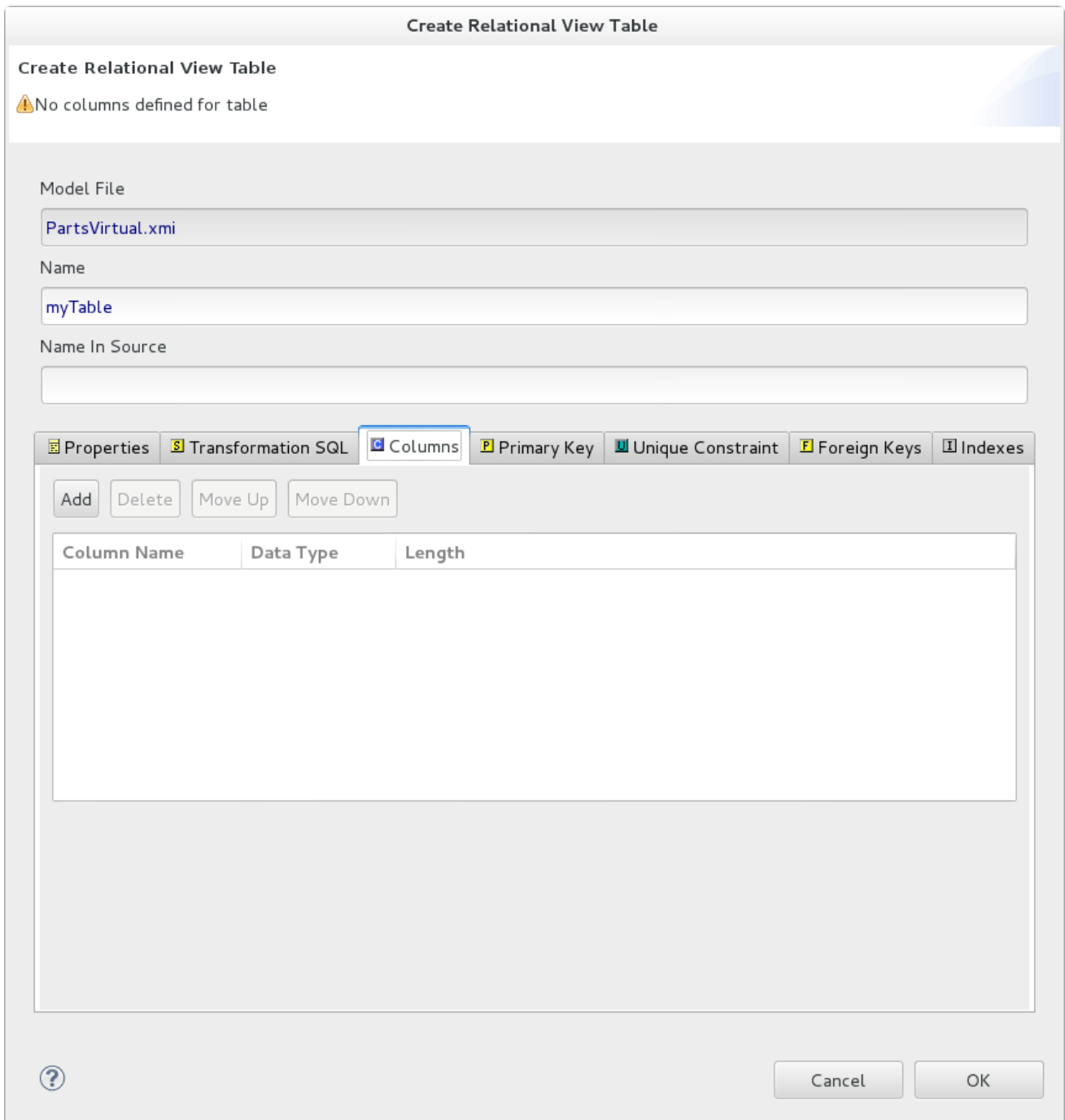
Figure 12.18. Columns Tab
