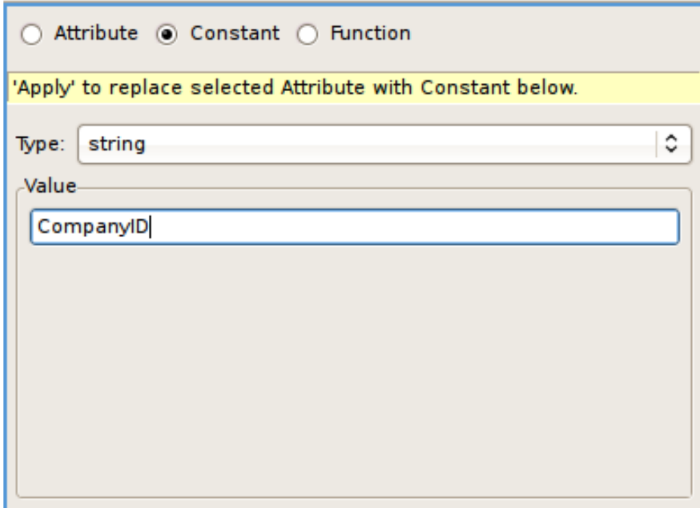
Figure 10.19. Constants Panel
