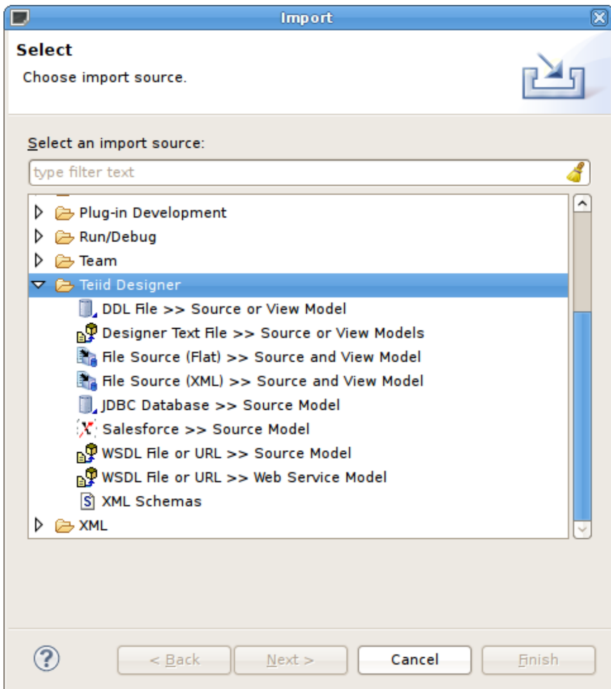
Figure 9.1. Import Wizard
