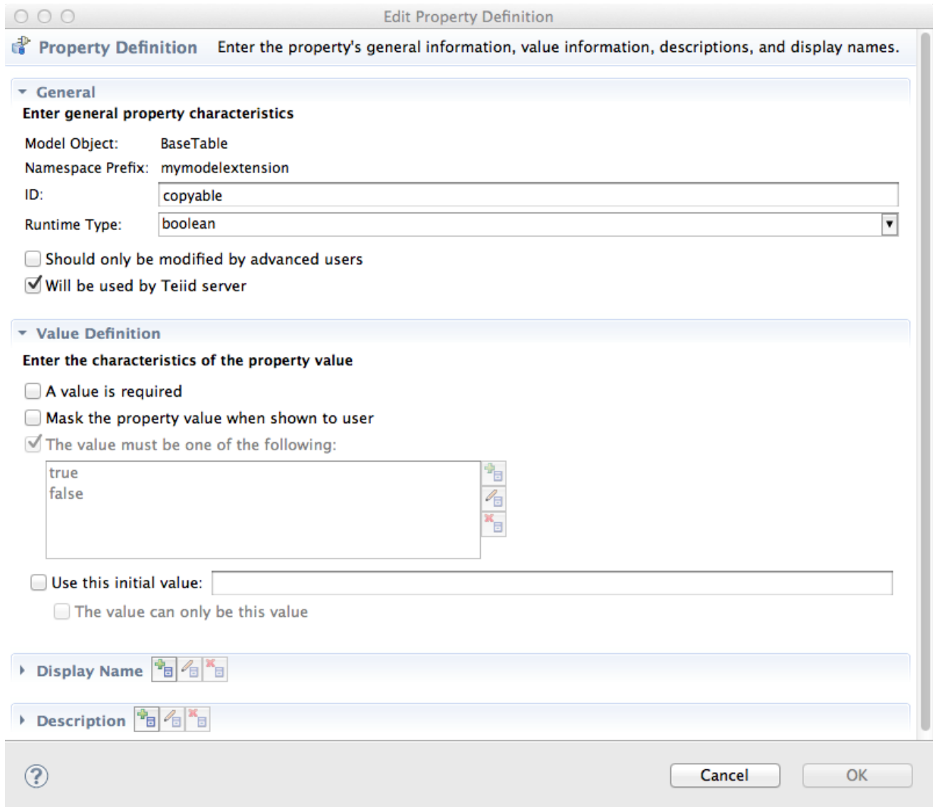
Figure 10.37. Edit Property Definition Dialog
