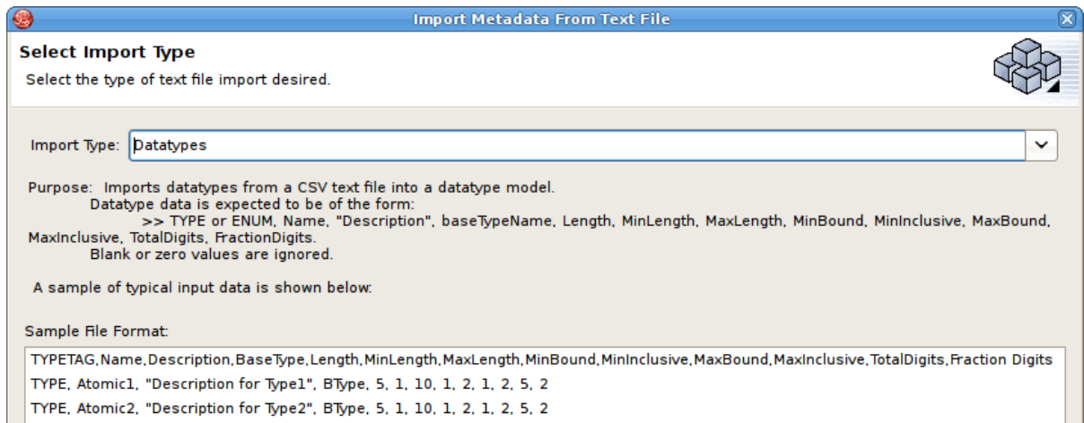
Figure 9.37. Select Import Type - Datatypes (CSV Format)
