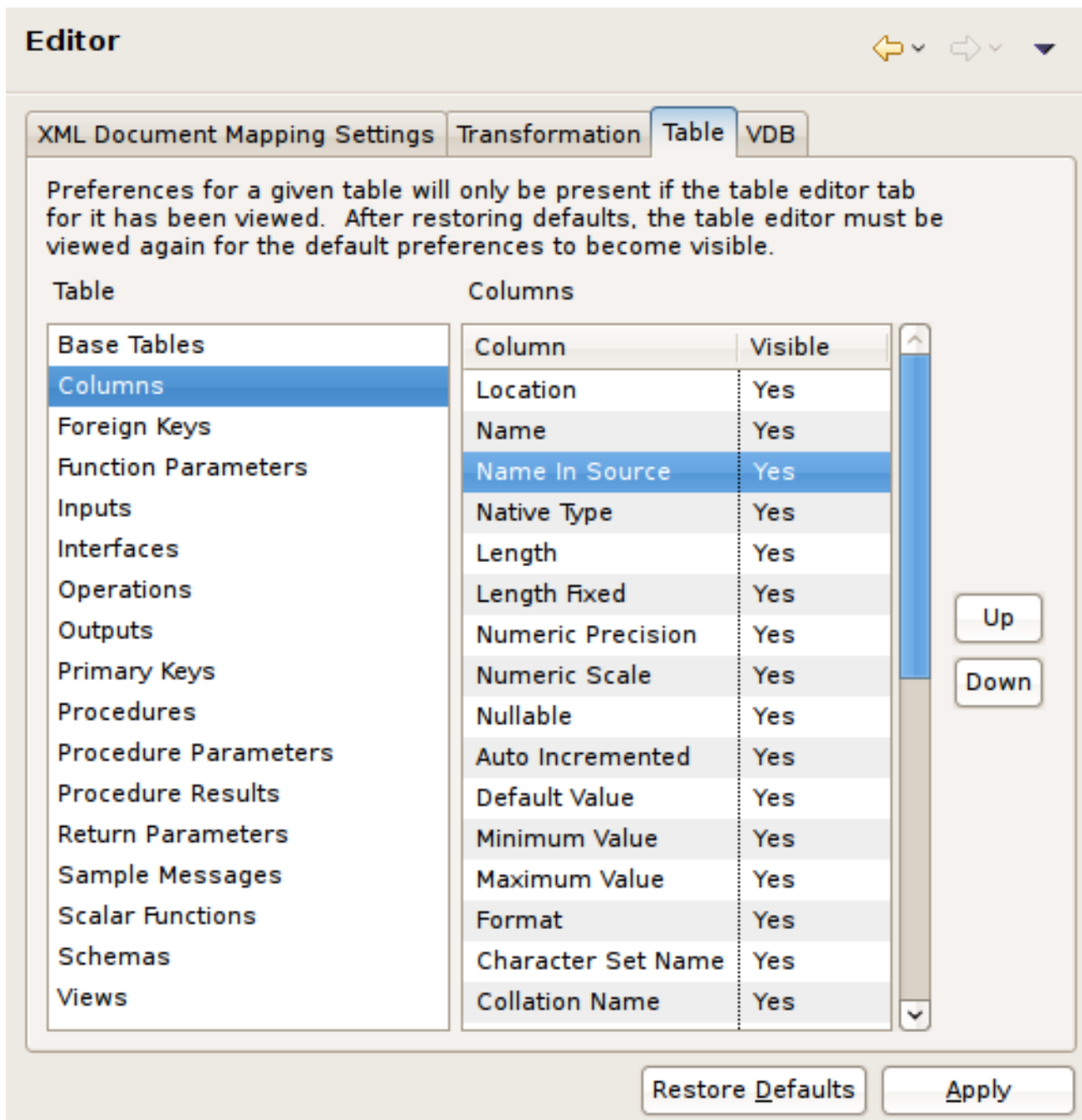
Figure B.6. Table Editor Preferences Panel
