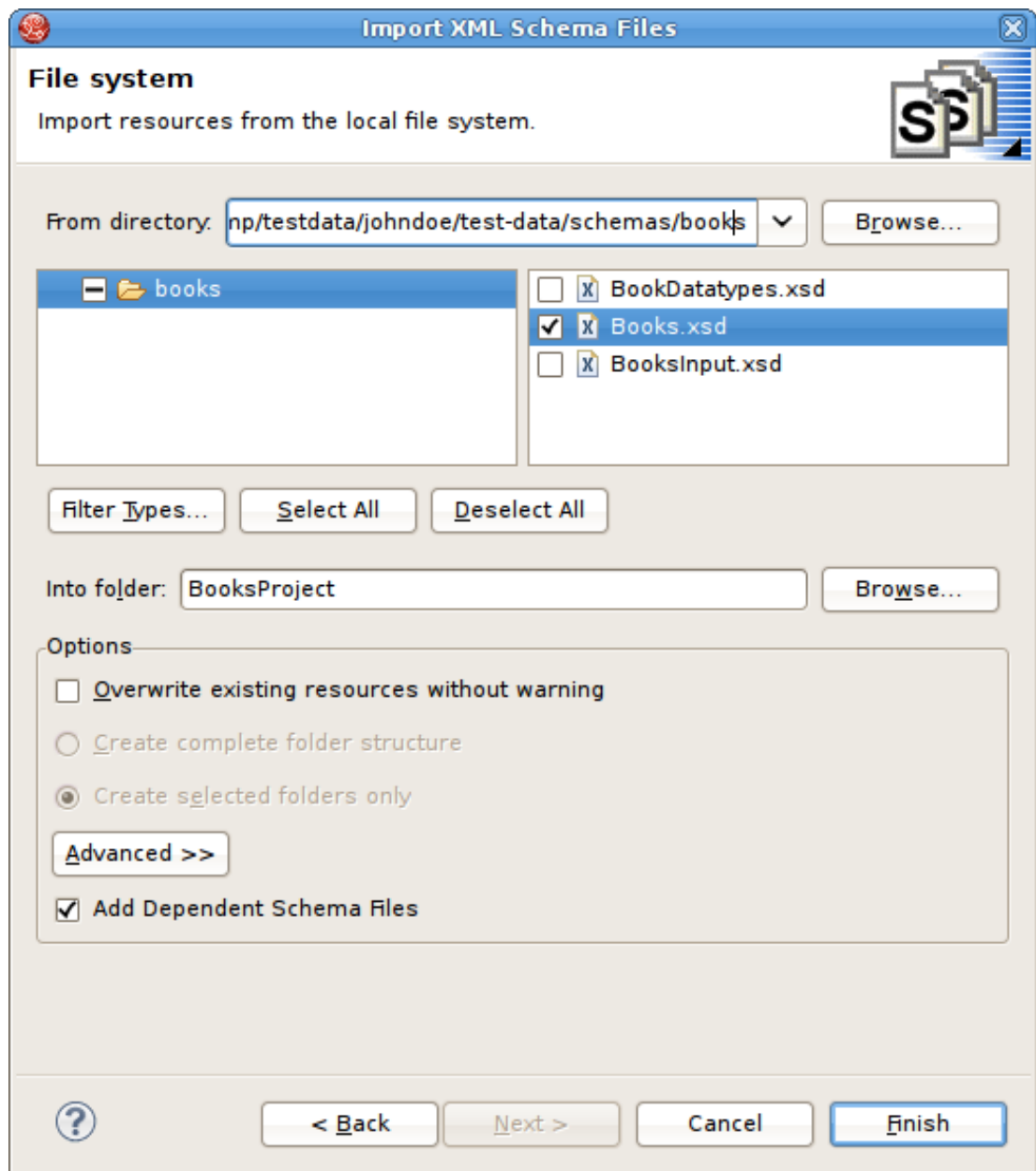
Figure 9.62. Select XSD From File System
