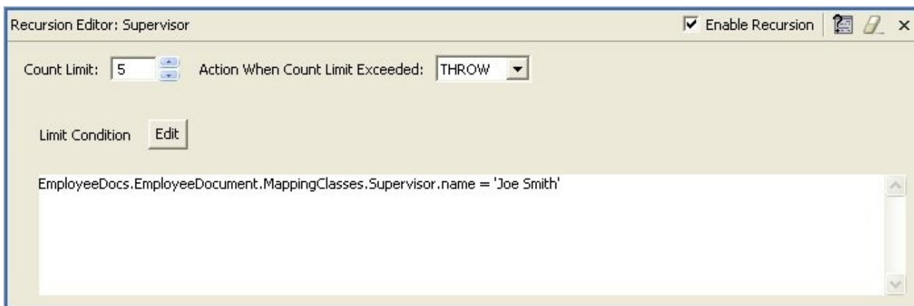
Figure 10.31. Recursion Editor
