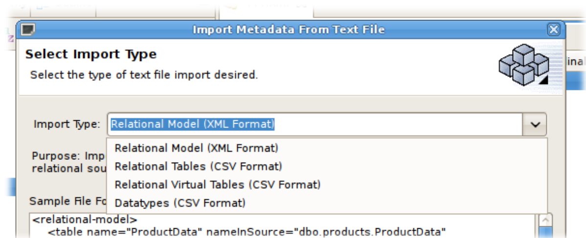
Figure 9.29. Import Wizard
