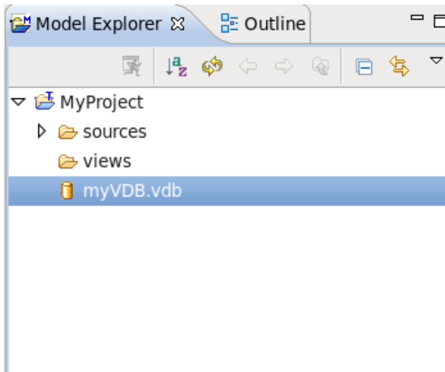
Figure 7.15. Model Explorer
