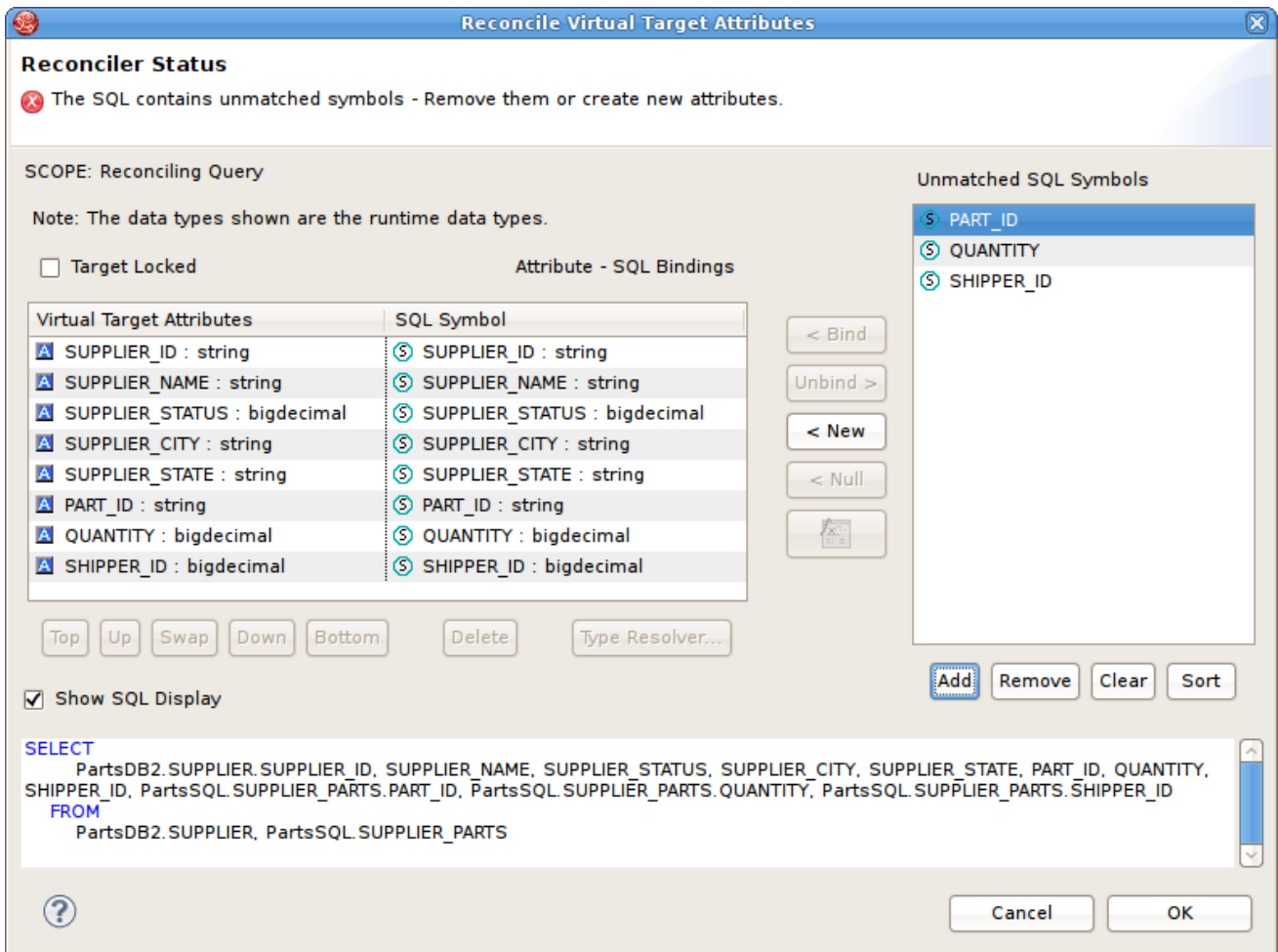
Figure 10.15. Reconciler Dialog
