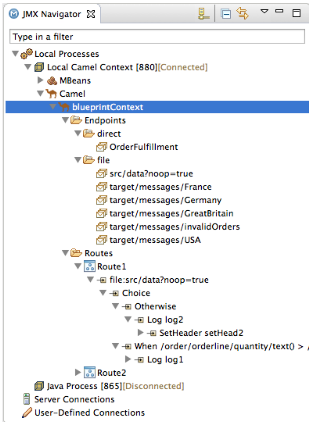
Figure 20.1. JMX Navigator view
