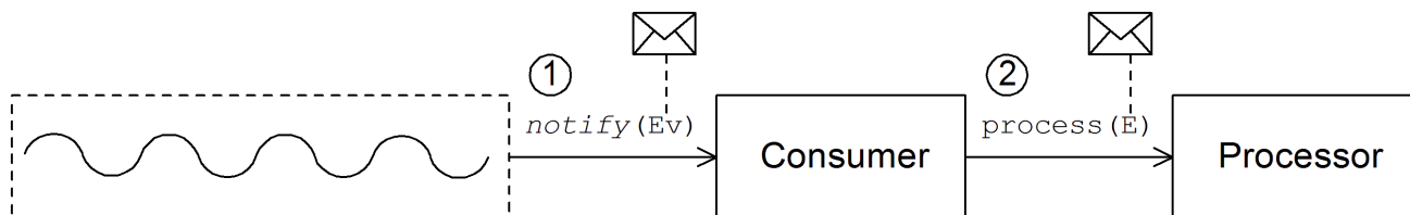
Figure 38.3. Event-Driven Consumer
