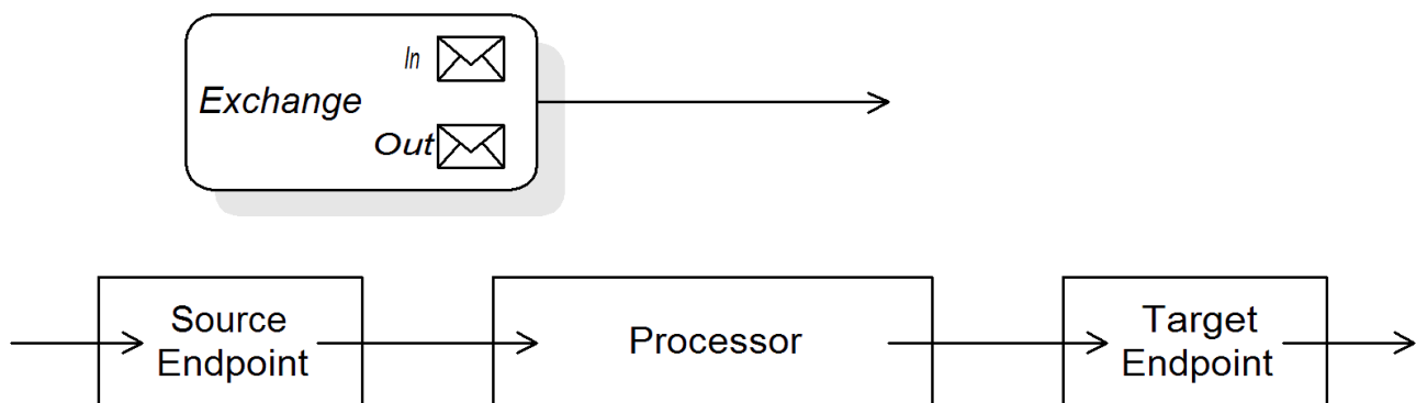
Figure 34.1. Exchange Object Passing through a Route
