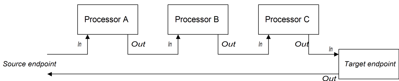
Figure 35.1. Pipelining Model
