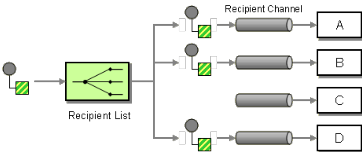
Figure 8.9. Multicast Pattern
