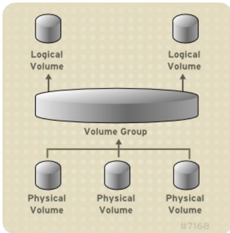
Figure 2.1. LVM Logical Volume Components
