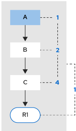
Figure 2.2. Example 1: Single rule
