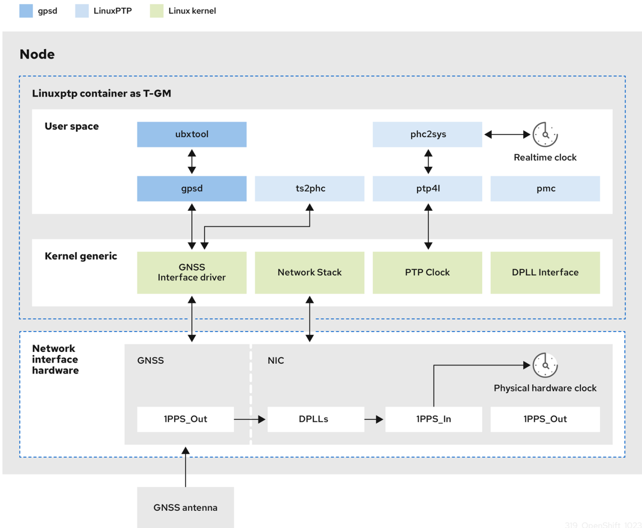
Figure 19.3. Overview of Synchronization with GNSS and T-GM
