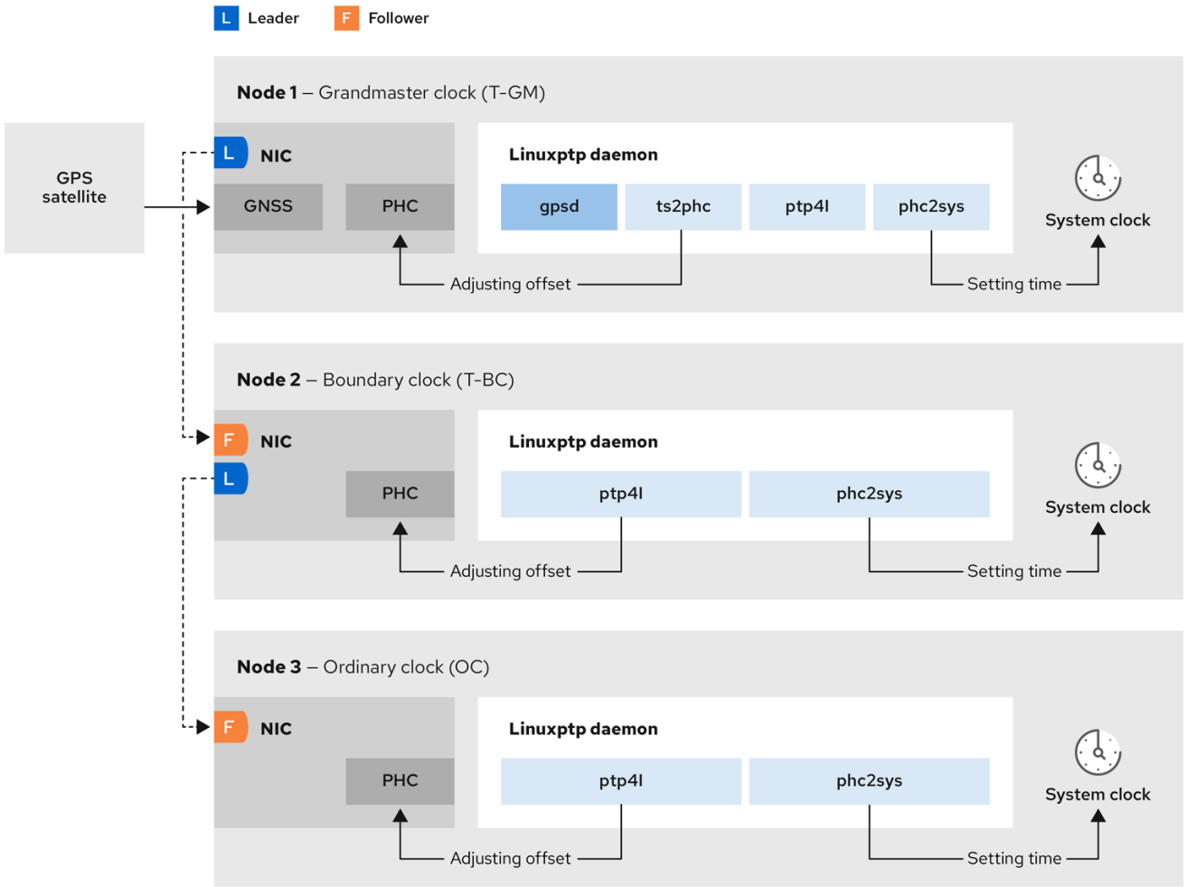
Figure 19.1. PTP nodes in the network
