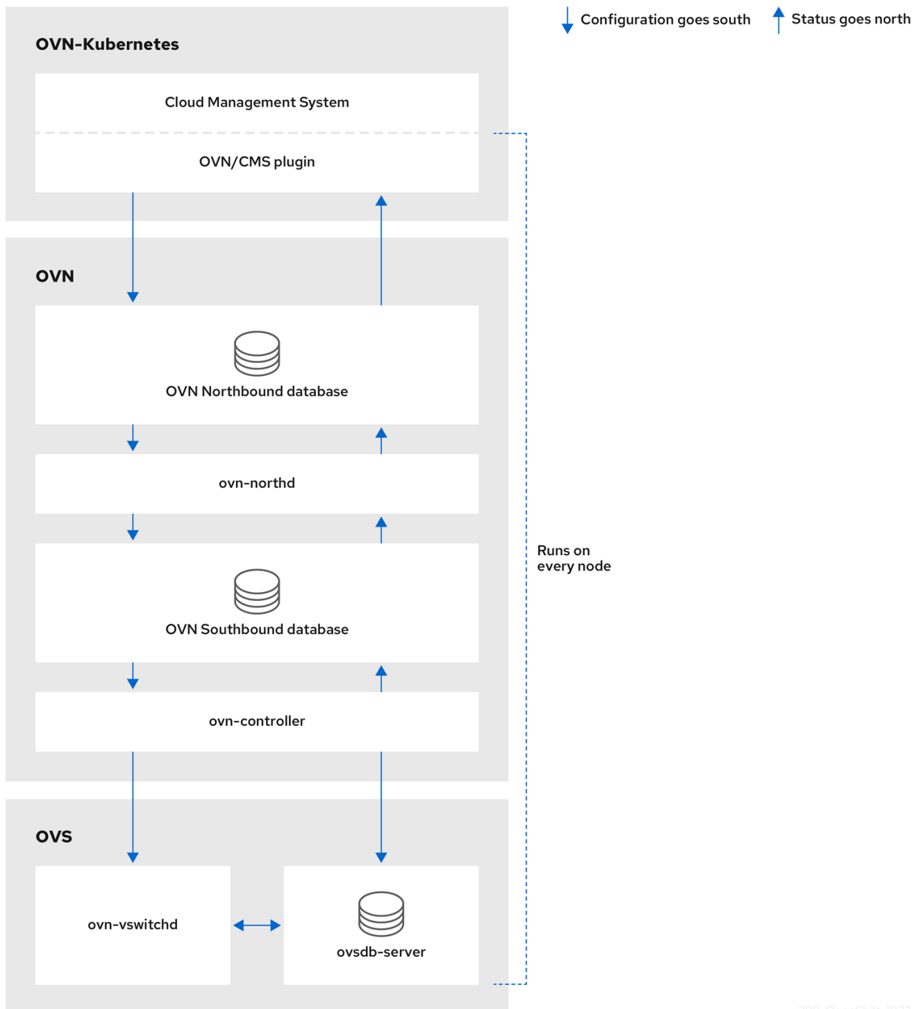
Figure 26.1. OVK-Kubernetes architecture
