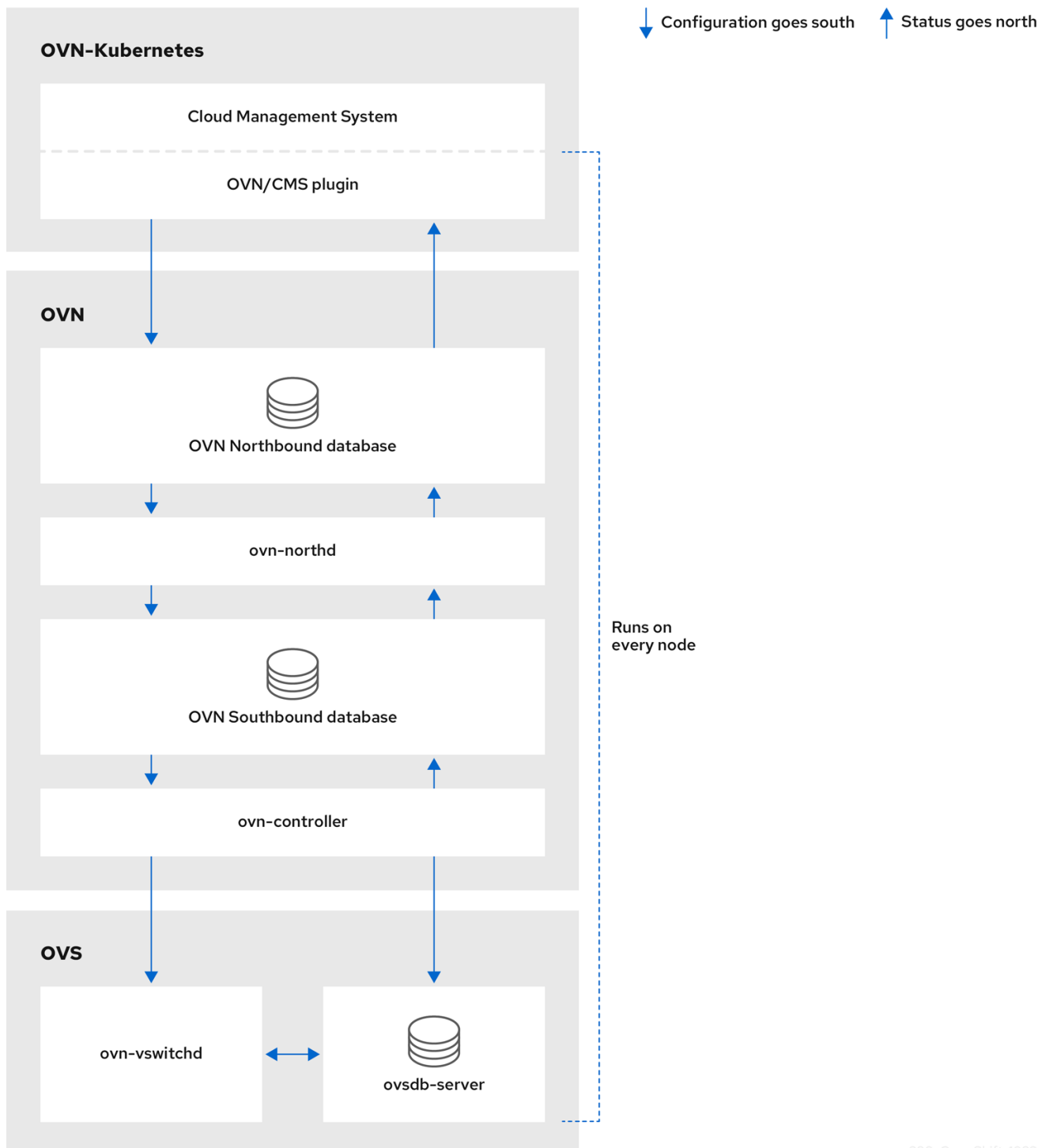
Figure 26.1. OVK-Kubernetes architecture
