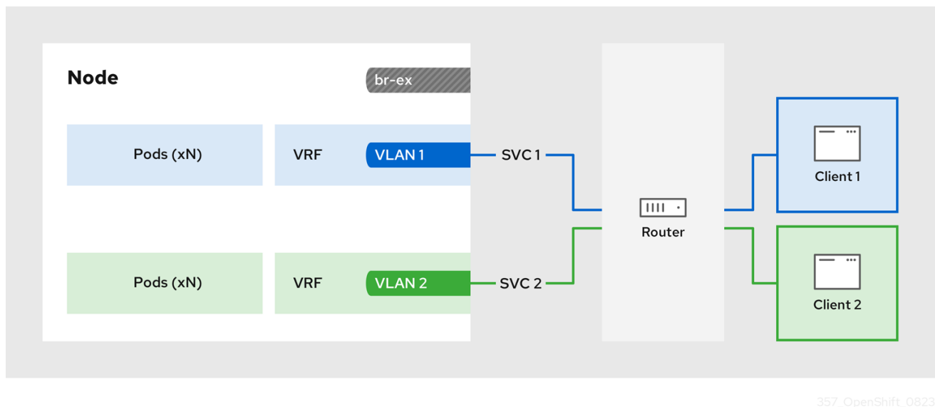
Figure 34.2. Network overview of managing symmetric routing by using VRFs with MetalLB
