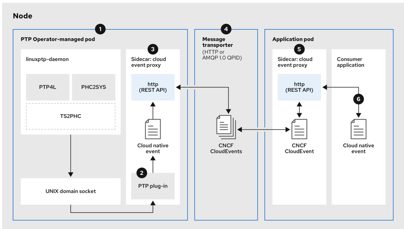
Figure 19.4. Overview of PTP fast events
