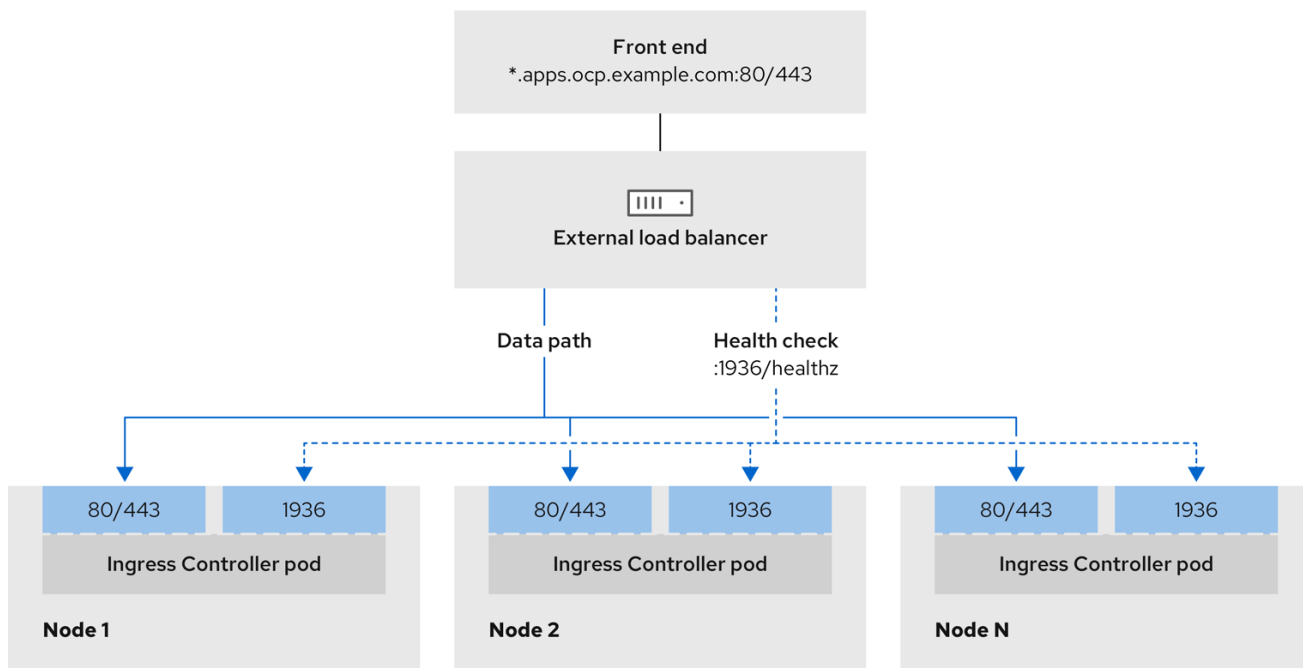
Figure 23.7. Example network workflow that shows an Ingress Controller operating in an OpenShift Container Platform environment
