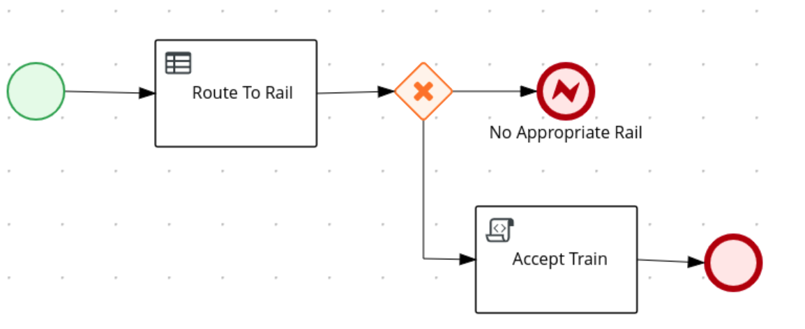
Figure 17.4. Example Accept Train business process with a DMN service
