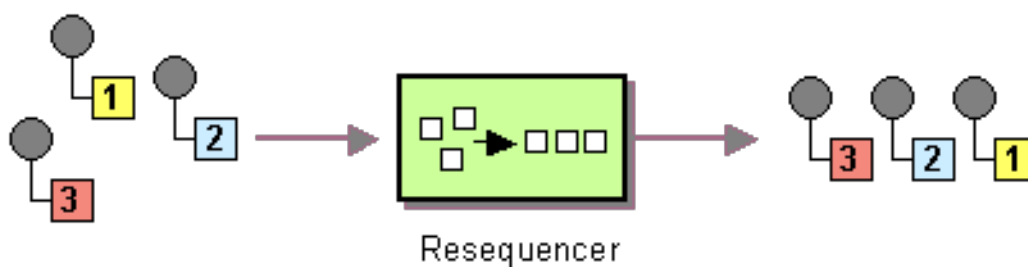
Figure 8.7. Resequencer Pattern
