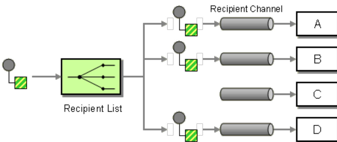
Figure 8.9. Multicast Pattern
