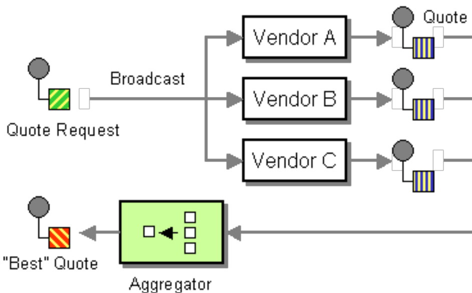
Figure 8.11. Scatter-Gather Pattern
