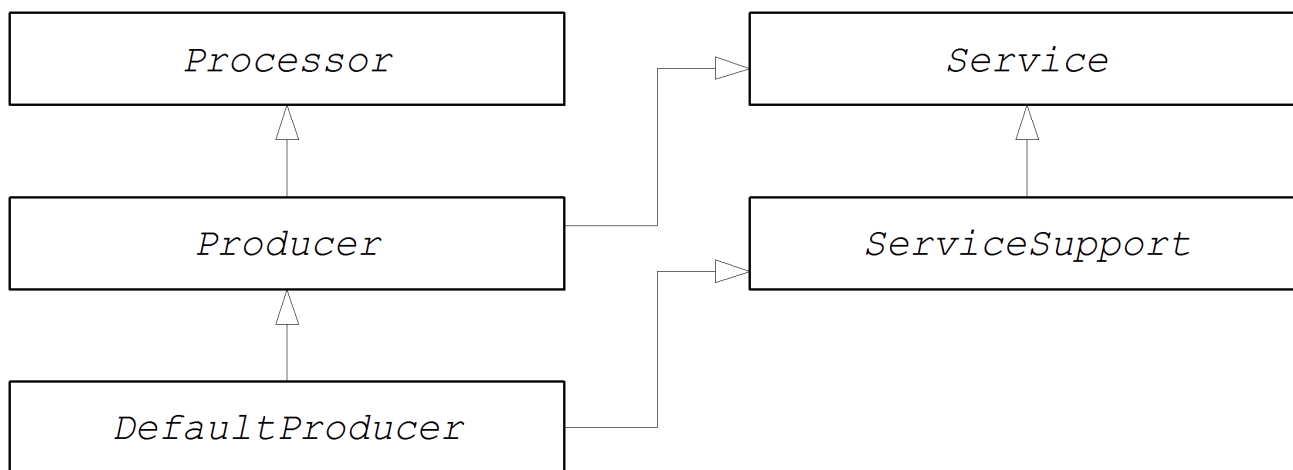
Figure 42.1. Producer Inheritance Hierarchy
