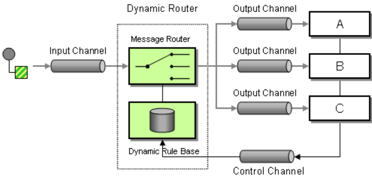
Figure 8.12. Dynamic Router Pattern
