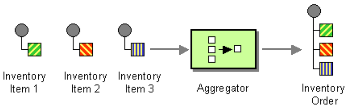
Figure 8.5. Aggregator Pattern
