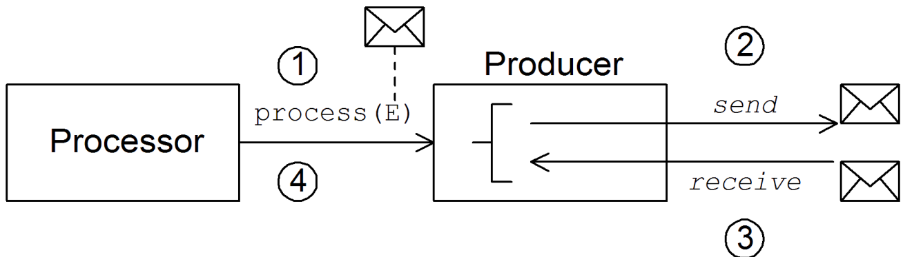
Figure 38.6. Synchronous Producer
