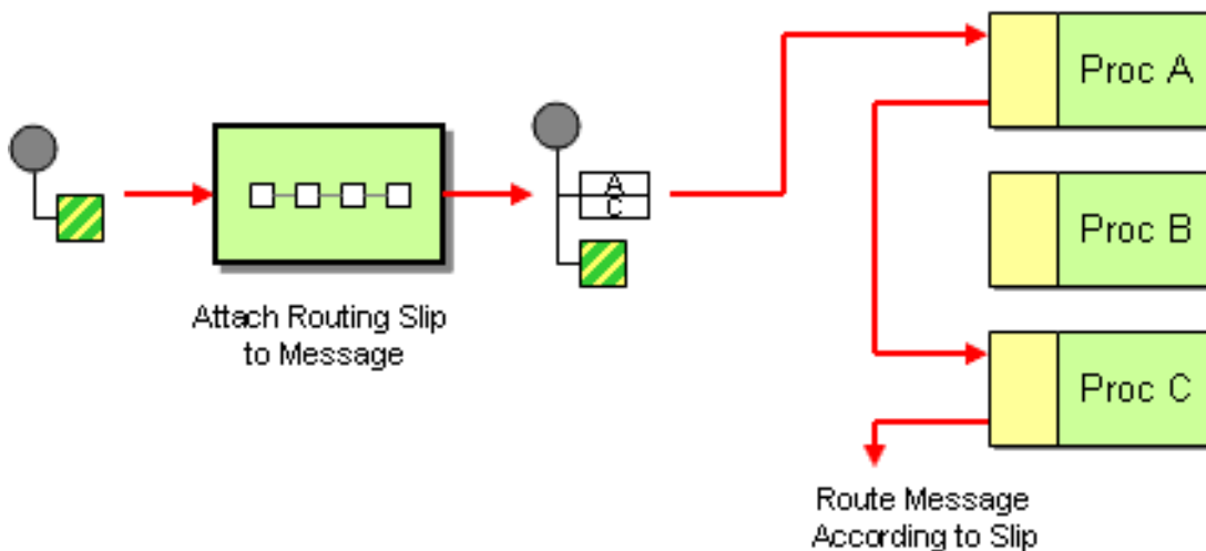
Figure 8.8. Routing Slip Pattern
