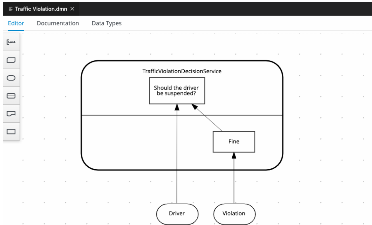
Figure 21.1. Example TrafficViolationDecisionService decision service with single-output decision
