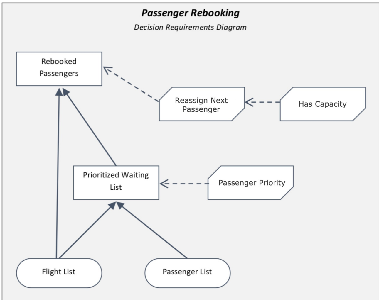
图2.1 Decision requirements diagram for passenger rebooking example
