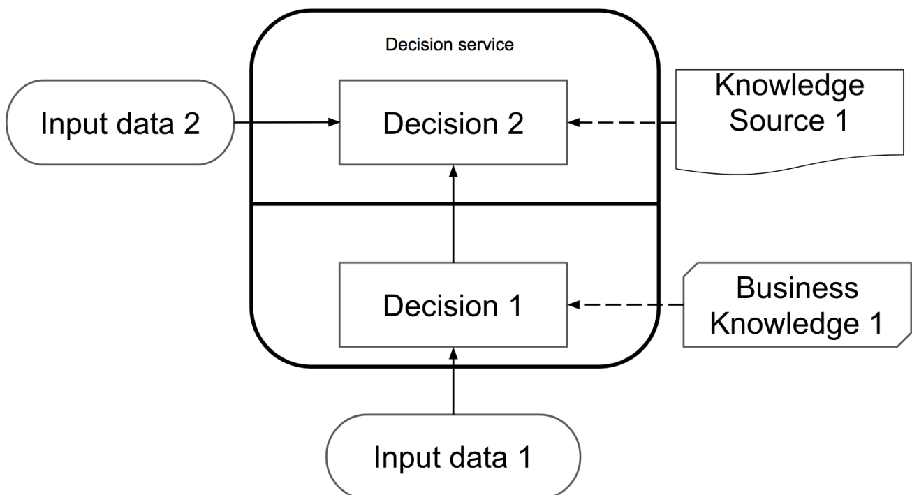
图1.1 Basic decision requirements diagram
