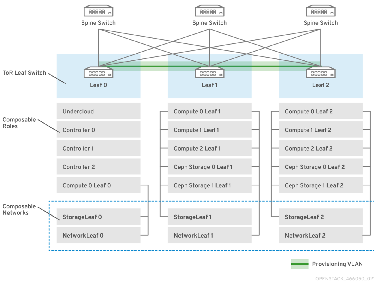
图3.1 VLAN provisioning network topology
