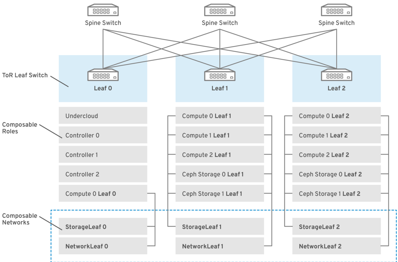
图1.1 Routed spine-leaf example
