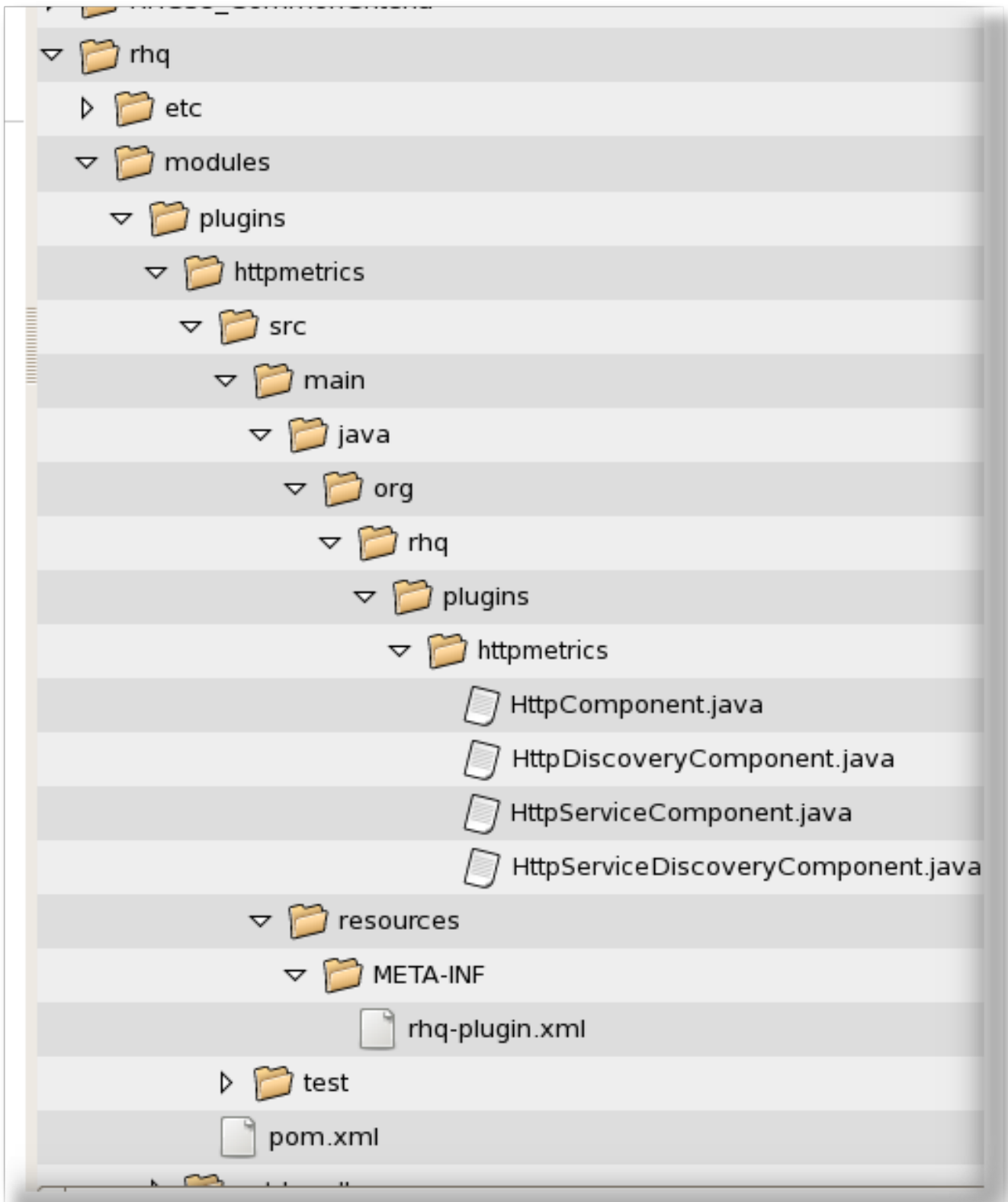
Figure 7. Directory Layout of an Agent Plug-in Project
