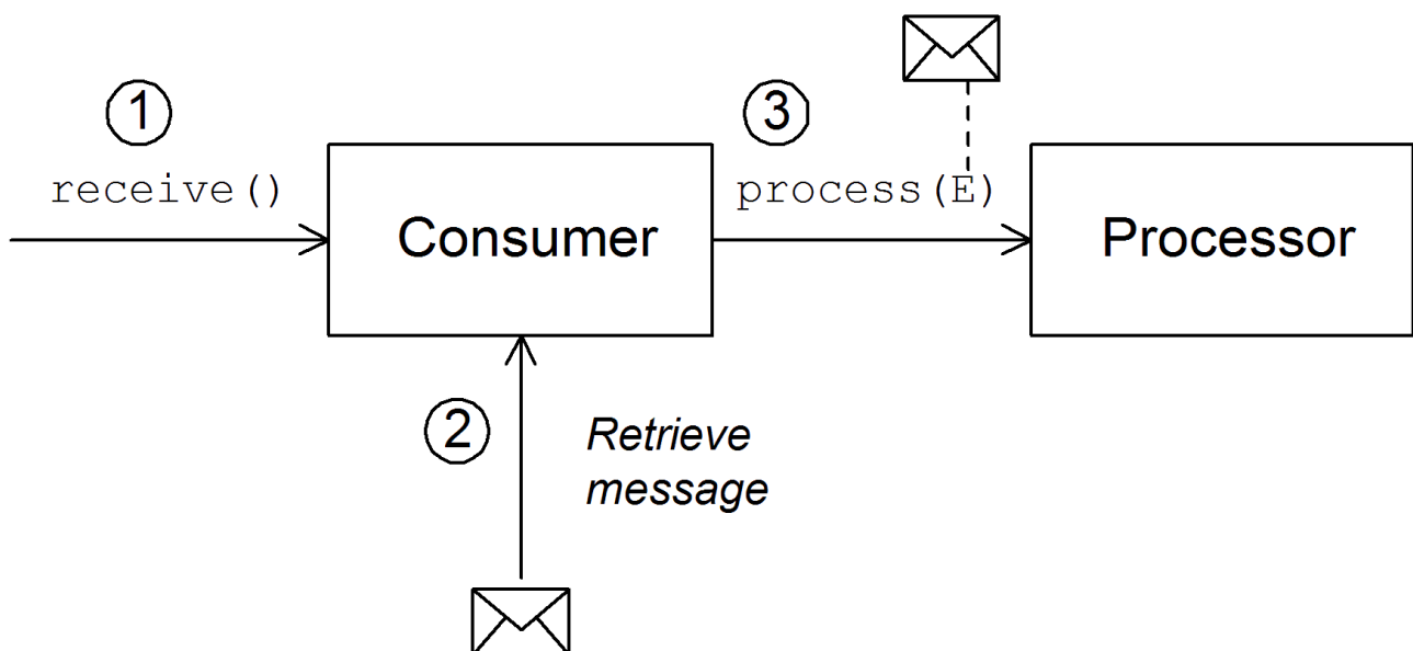
図38.5 Polling Consumer
