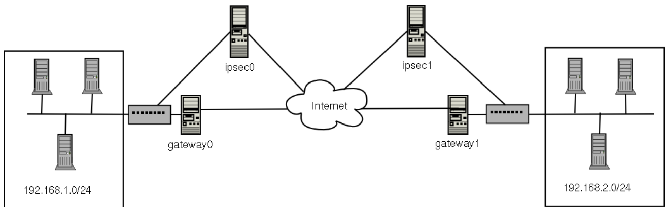
Figure 6.1. A Network-to-network IPsec tunneled connection
