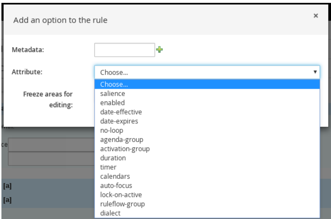
图4.10 Rule options
