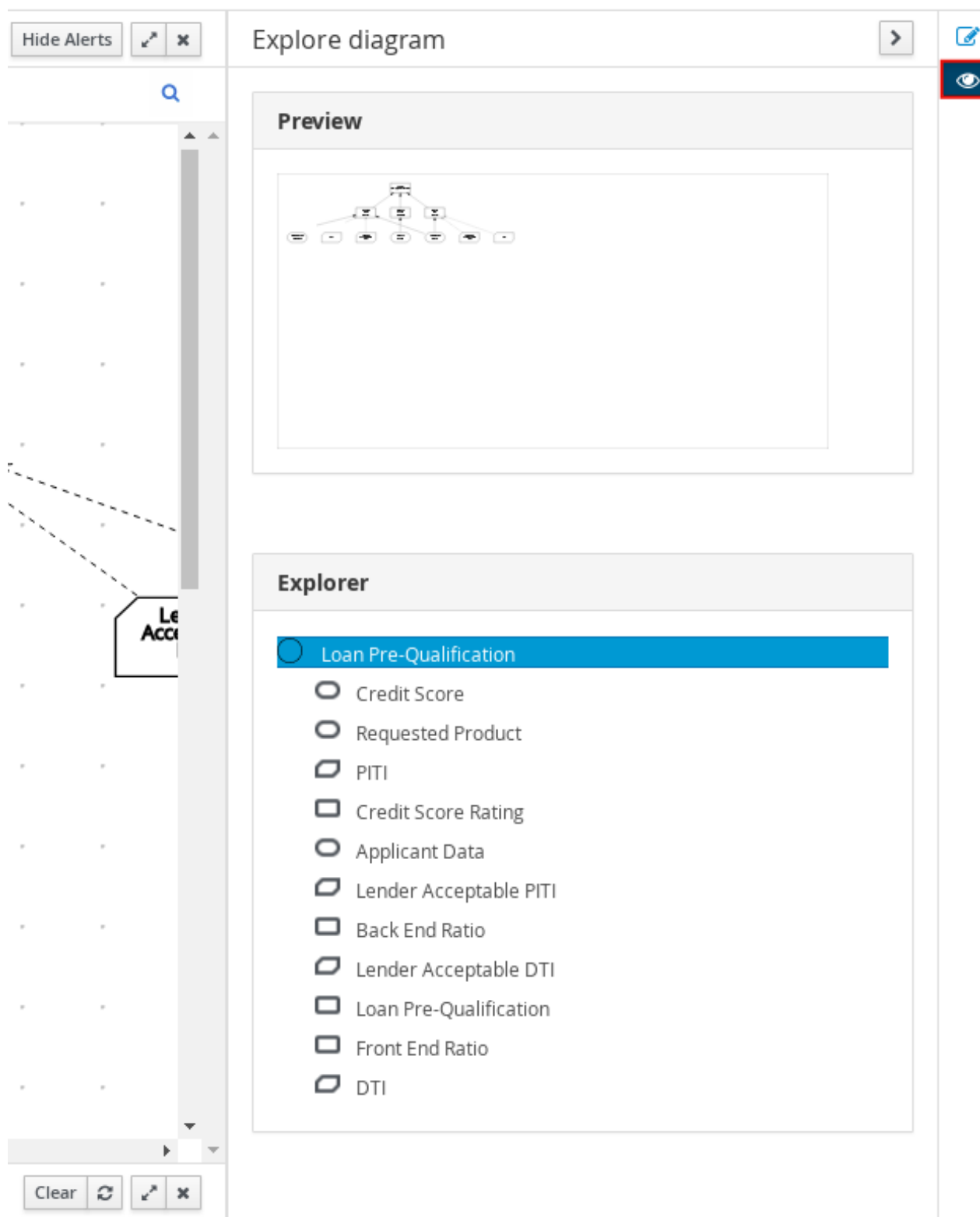
图3.49 Explore diagram view
