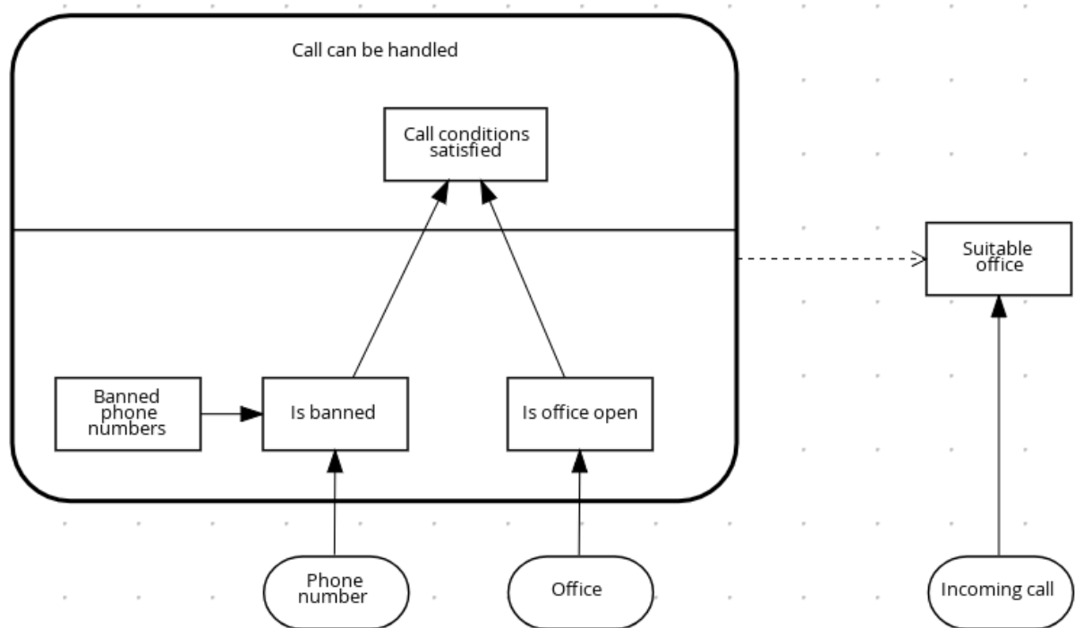
图3.10 Completed DRD for phone call handling with a decision service
