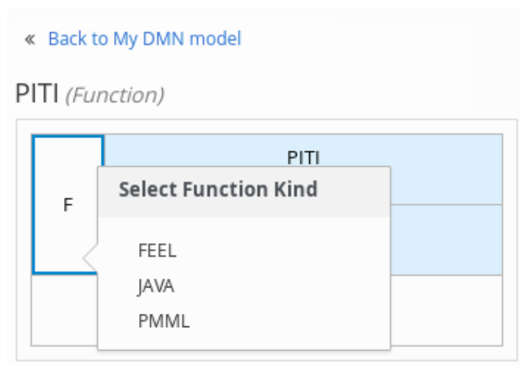
图3.5 Selecting the function or other logic type for a business knowledge model
