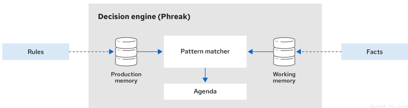
图1.1 Overview of basic decision engine components
