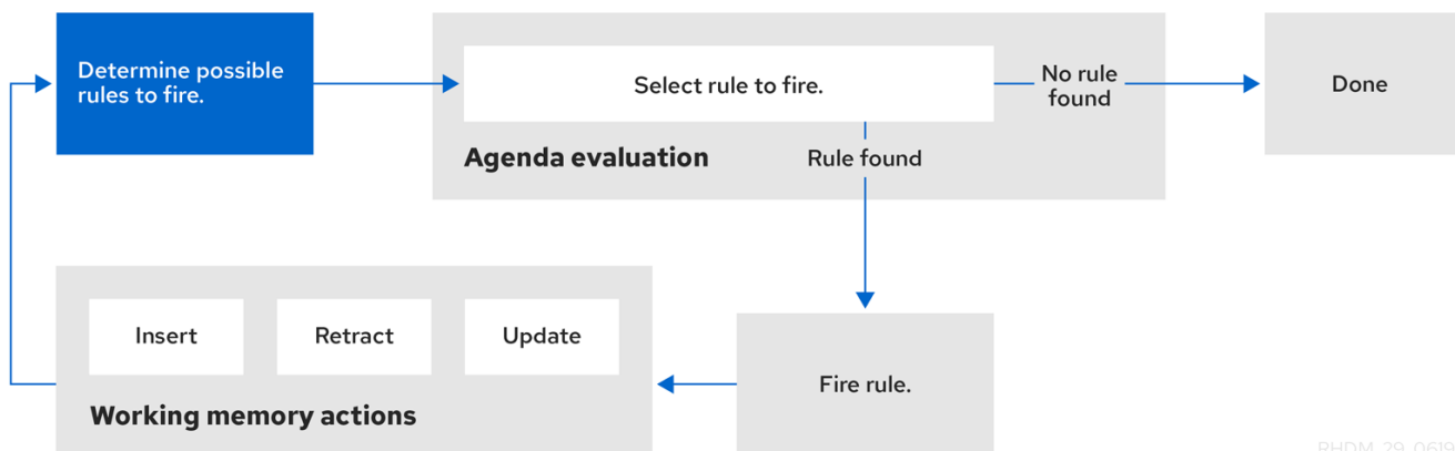
图 4.1 Two-phase execution process in the decision engine
