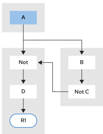
图5.5 Example 4: Single rule with a subnetwork and no pattern sharing
