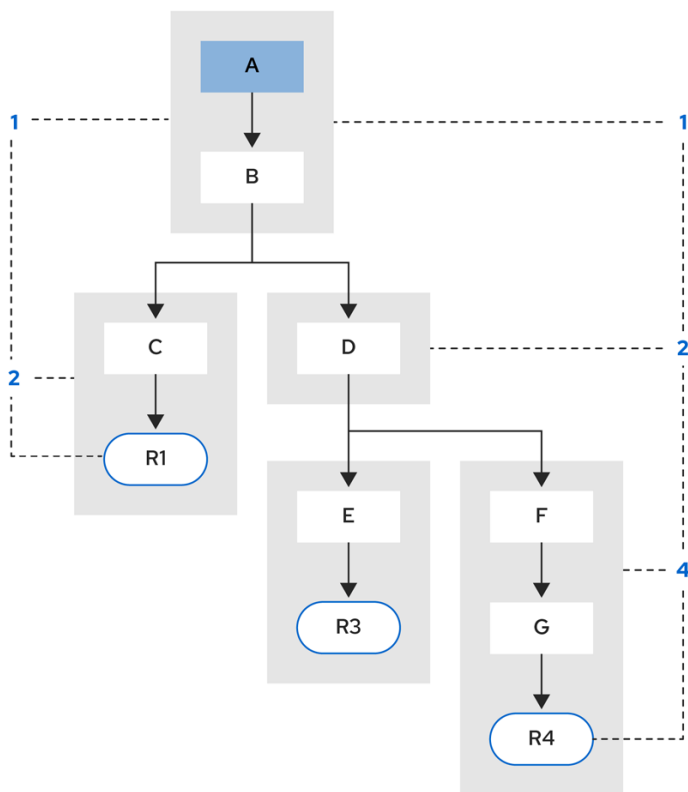
图5.4 Example 3: Three rules with pattern sharing
