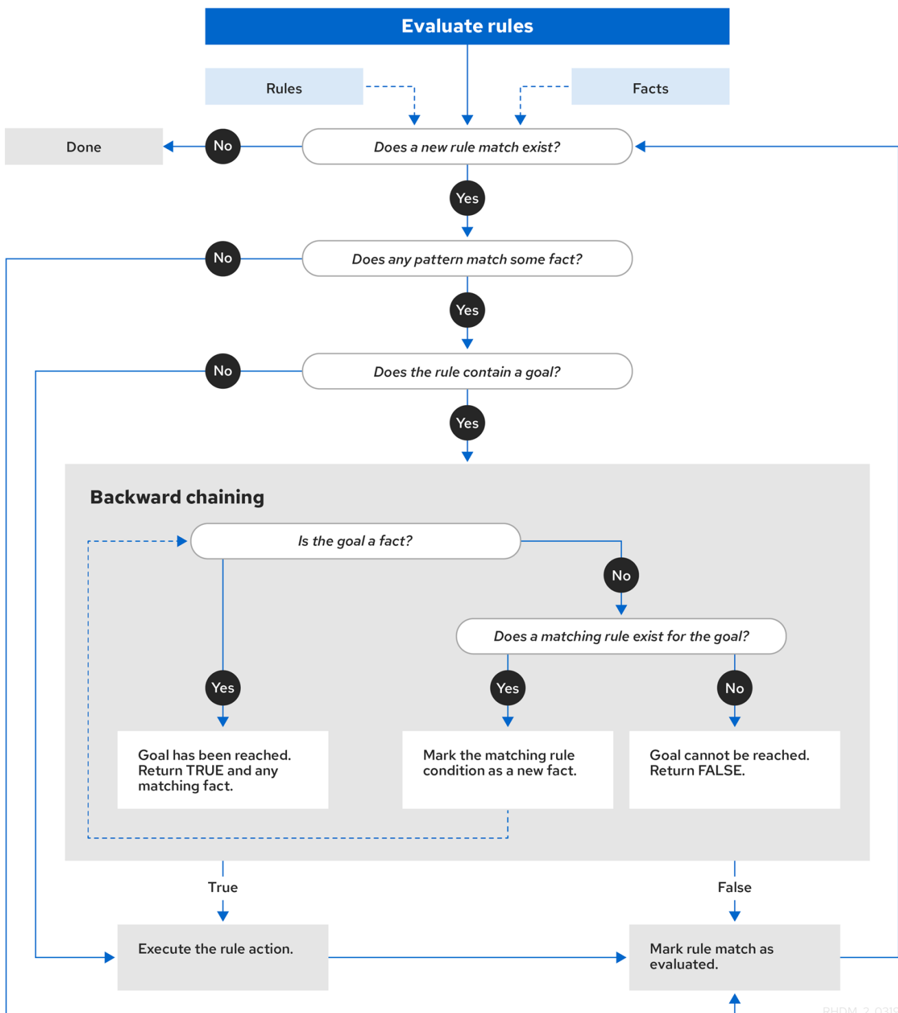
图5.7 Rule evaluation logic using forward and backward chaining
