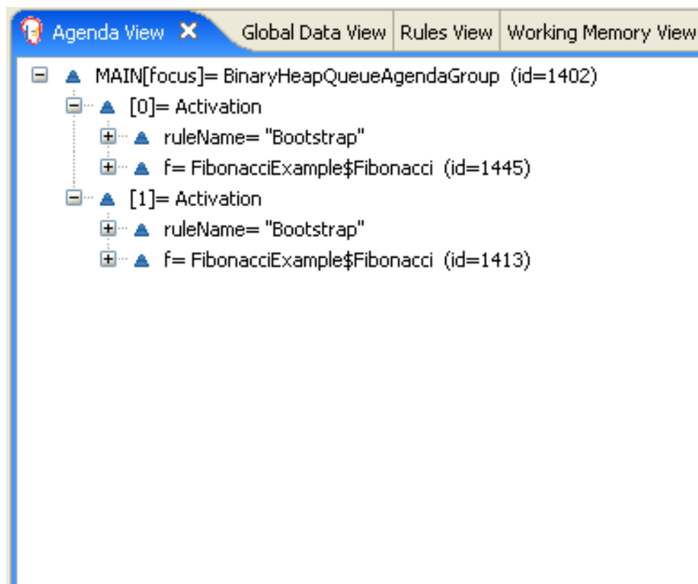
图7.9 Rules "Recurse" and "Bootstrap" in Agenda View 2
