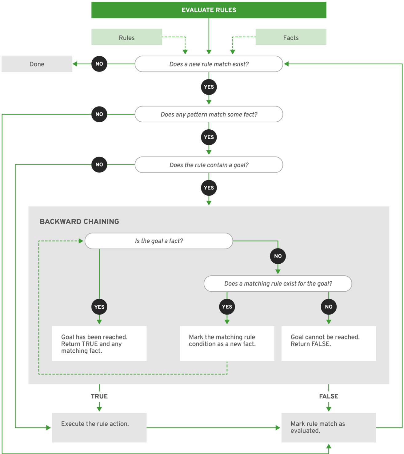
7.27 Rule evaluation logic using forward and backward chaining
