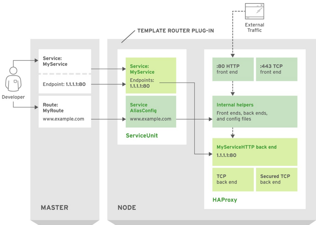
Figure 3.1. HAProxy Router Data Flow
