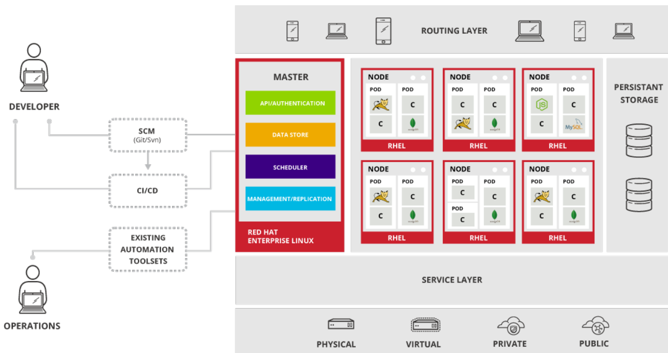
Figure 1.1. OpenShift Architecture Overview
