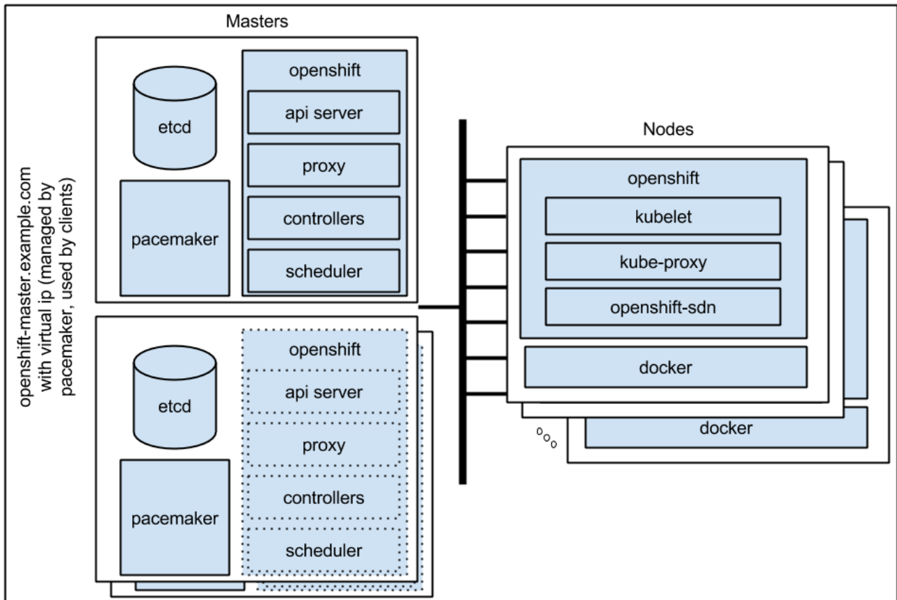
Figure 2.1. Highly-available Masters Using Pacemaker
