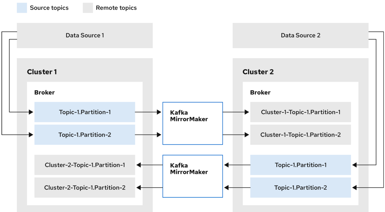
Figure 7.2. Bidirectional replication
