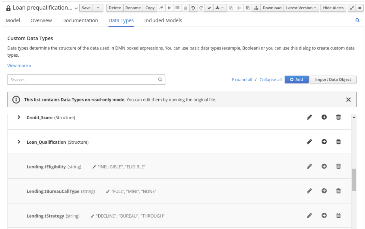
Figure 3.41. DMN file with data types from the included DMN model
