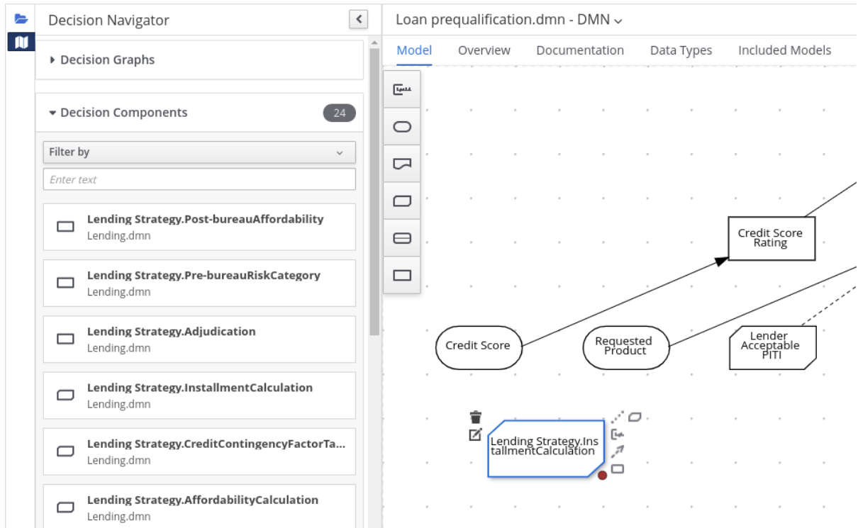
Figure 3.42. Adding DRD components from the included DMN model
