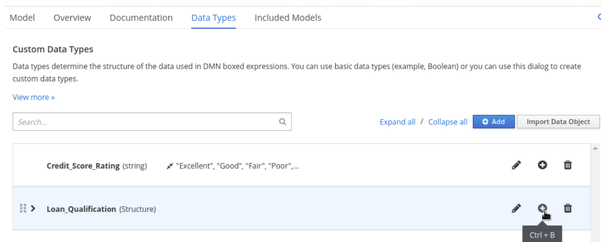
Figure 3.32. Adding a new structured data type with nested fields
