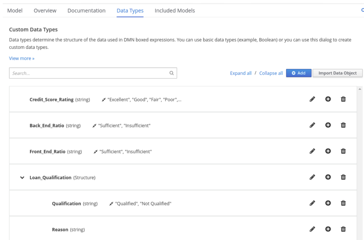
Figure 3.33. Adding nested data types with constraints
