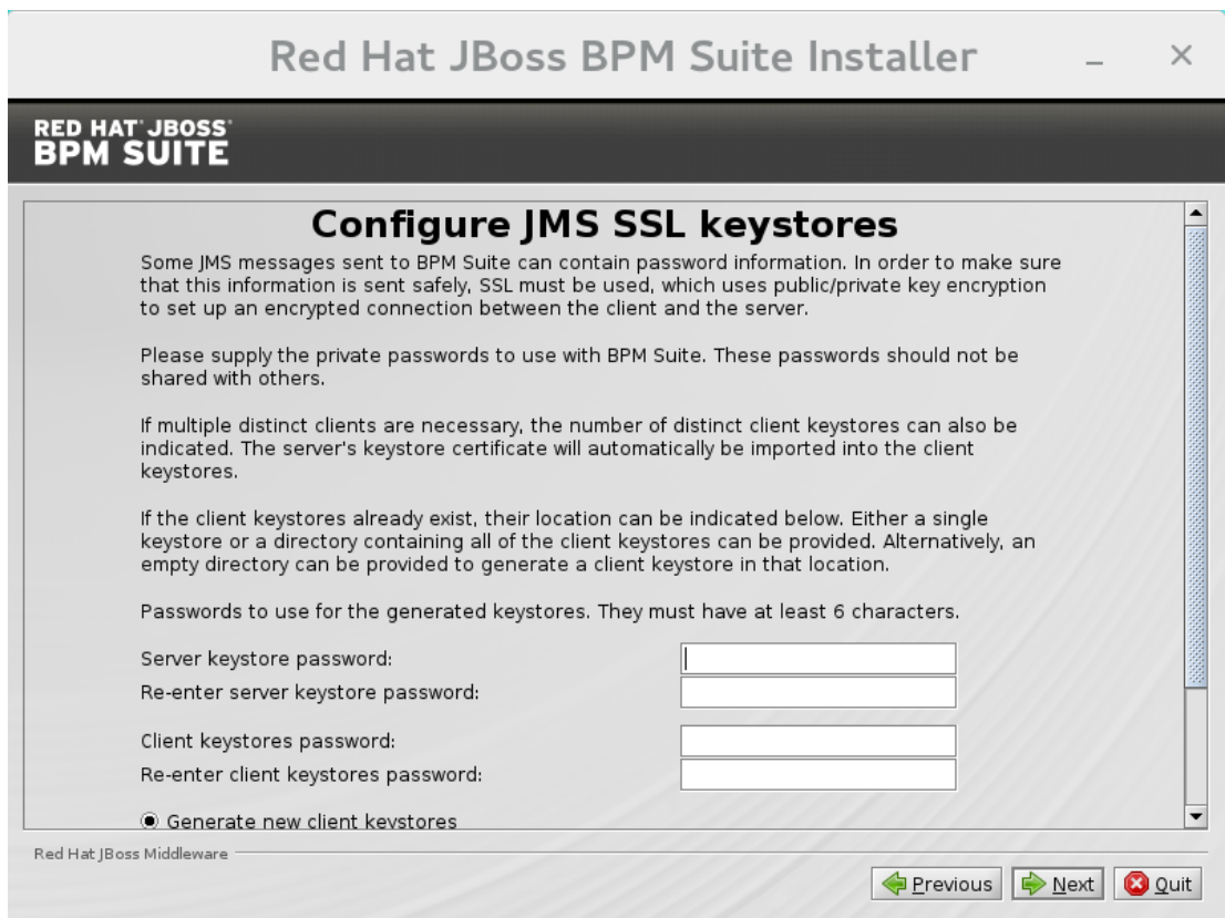
Figure 3.10. Configuring JMS SSL Keystores
