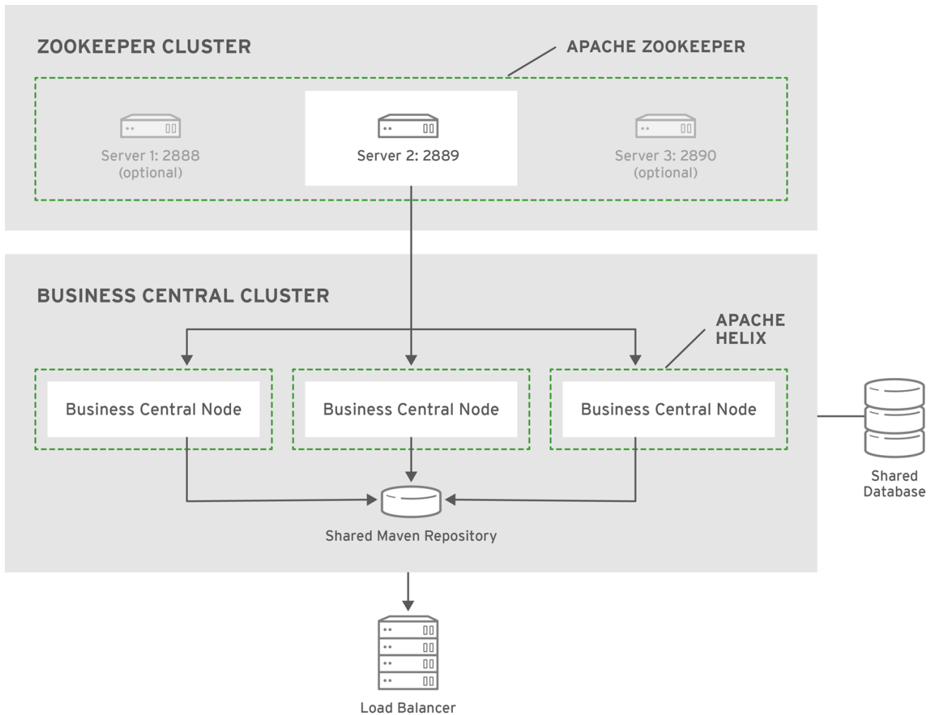
Figure 6.1. Schema of Red Hat JBoss BPM Suite Cluster
