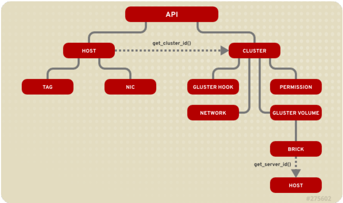
Figure 16.1. Object Hierarchy
