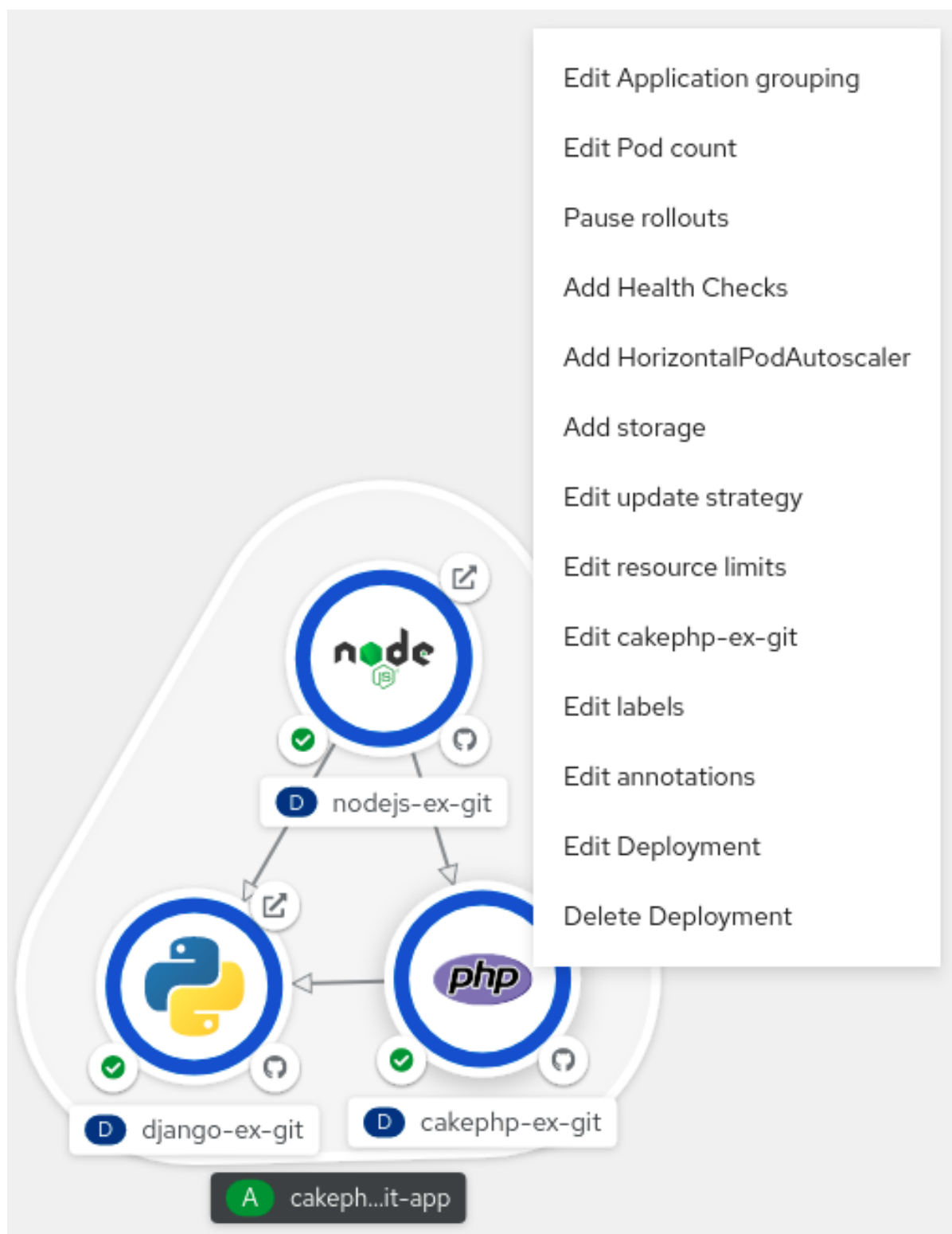
Figure 4.7. Deleting deployment option
