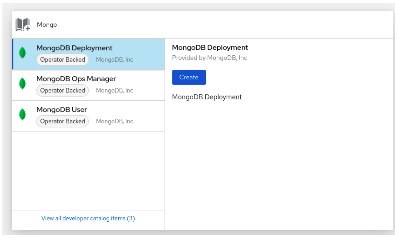
Figure 4.3. Adding component via quick search
