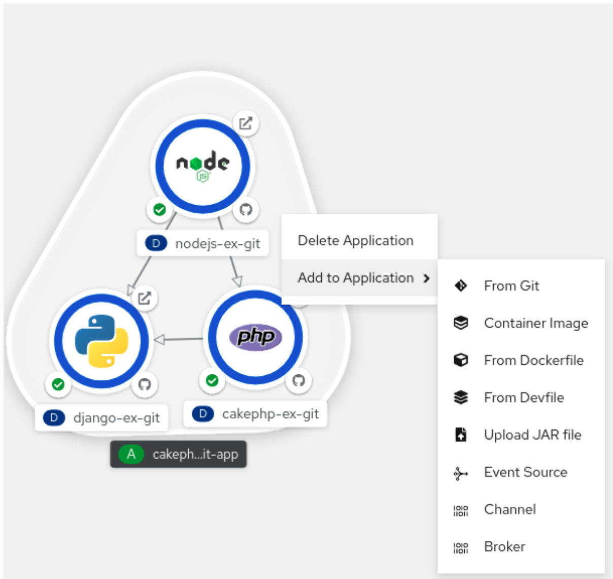
Figure 4.6. Add resource context menu
