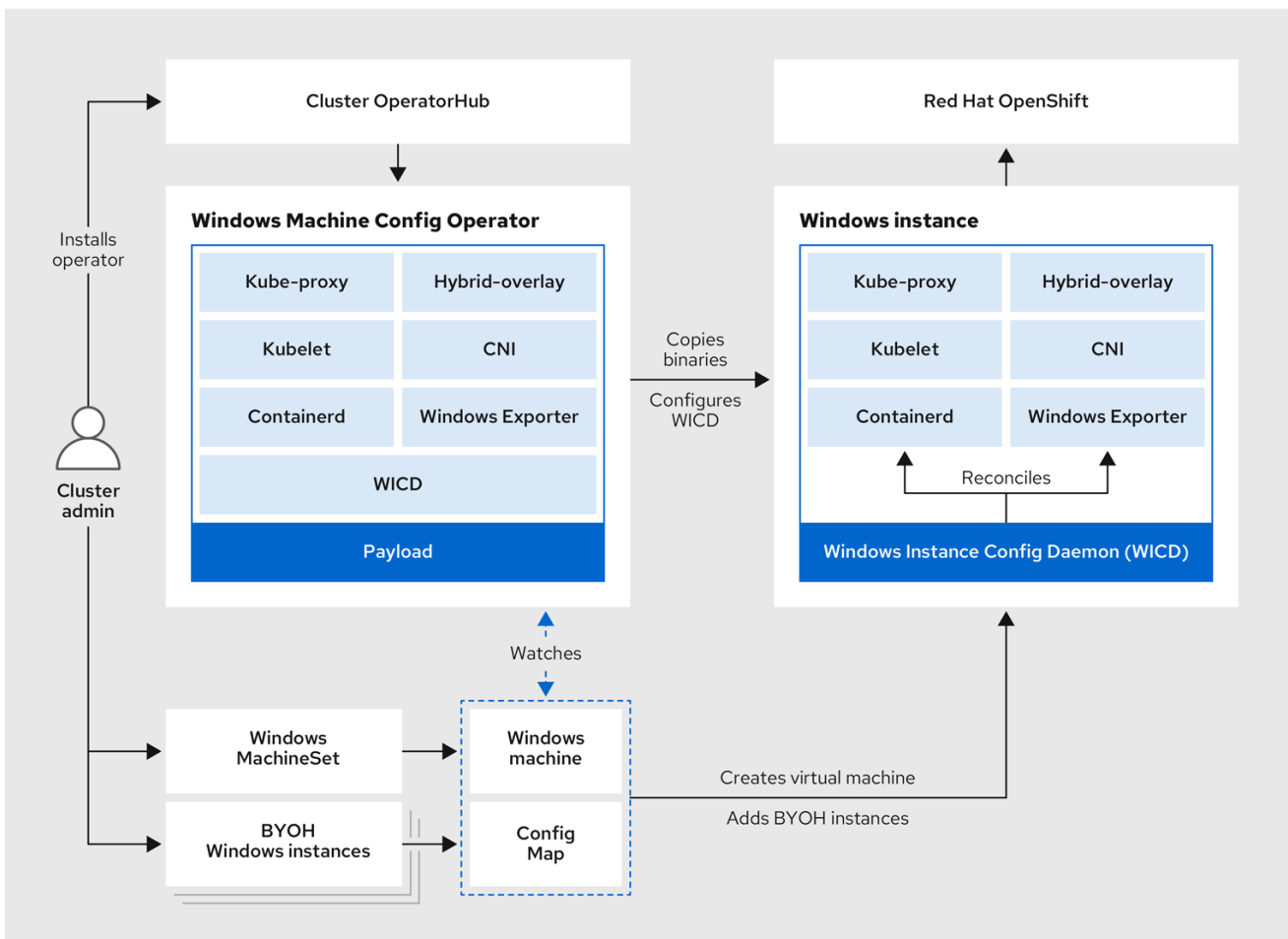
Figure 3.1. WMCO design
