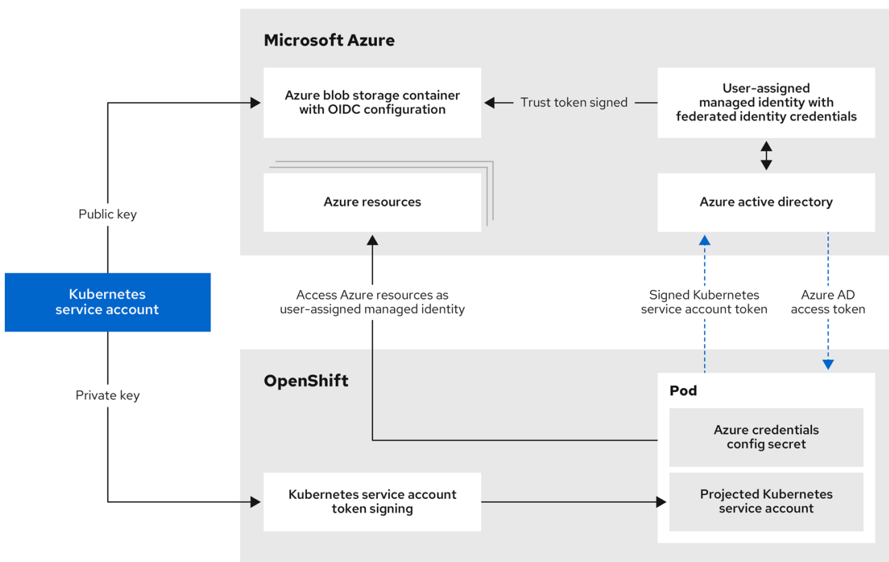
Figure 19.4. Azure AD Workload Identity authentication flow
