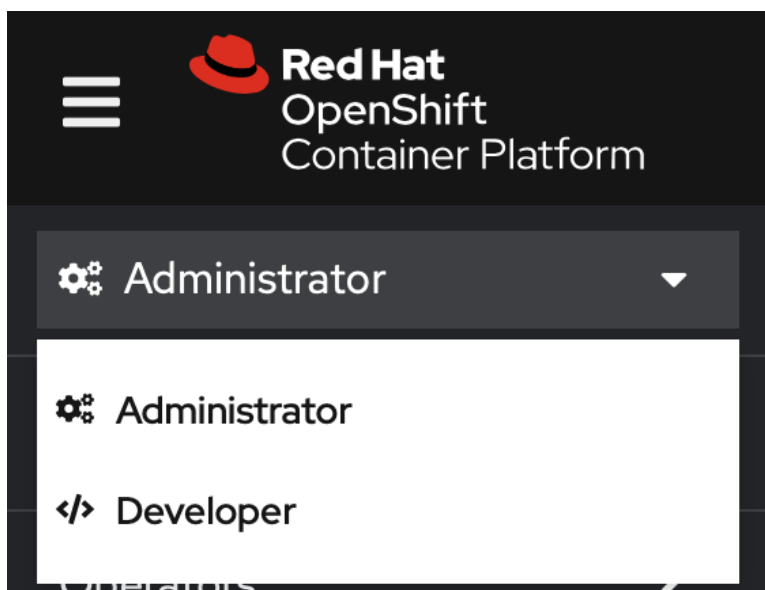
Figure 3.1. Perspective switcher
