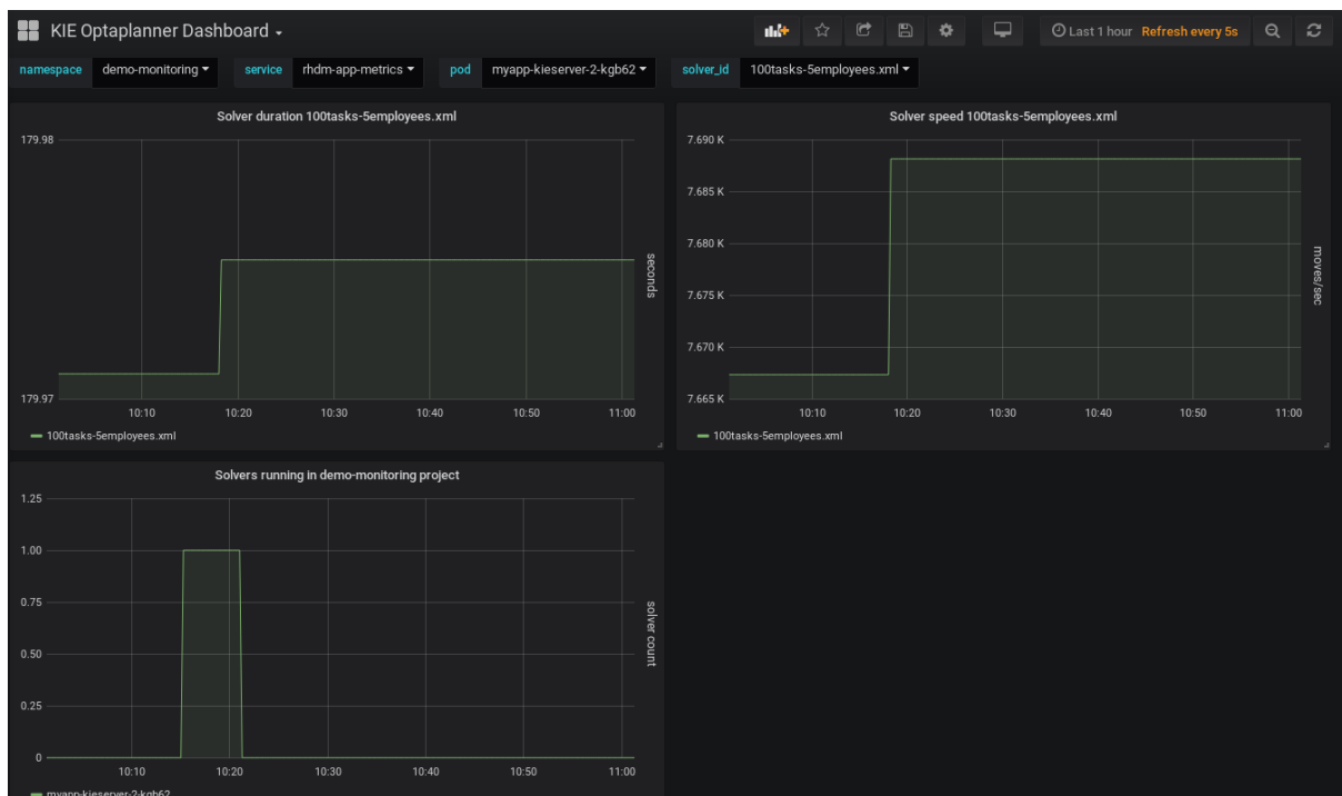
Figure 18.9. Grafana dashboard with KIE Server metrics for solvers
