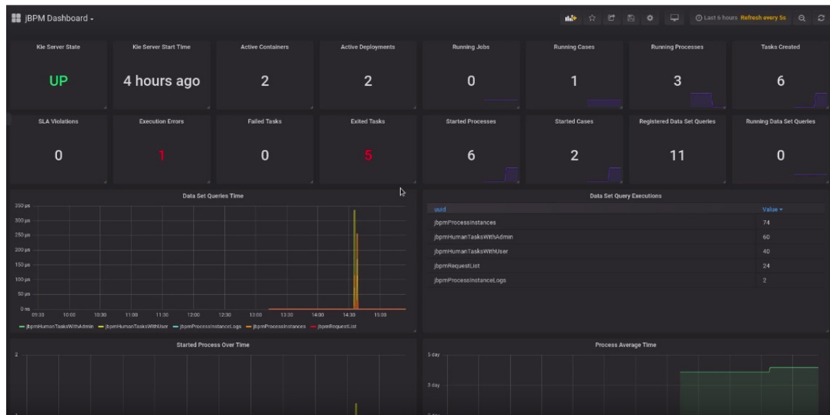
Figure 18.10. Grafana dashboard with KIE Server metrics for processes, cases, and tasks
