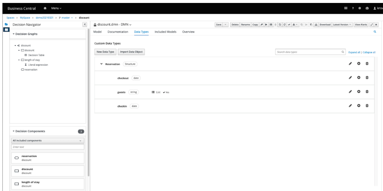
Figure 17.2. Example DMN model using specificItemDefinition structure
