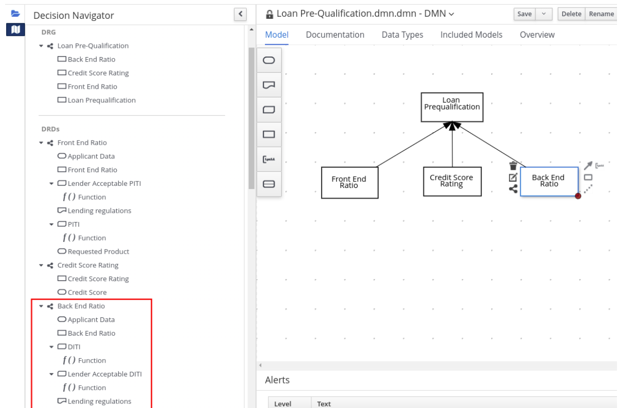
Figure 6.57. Overview of back end ratio DRD
