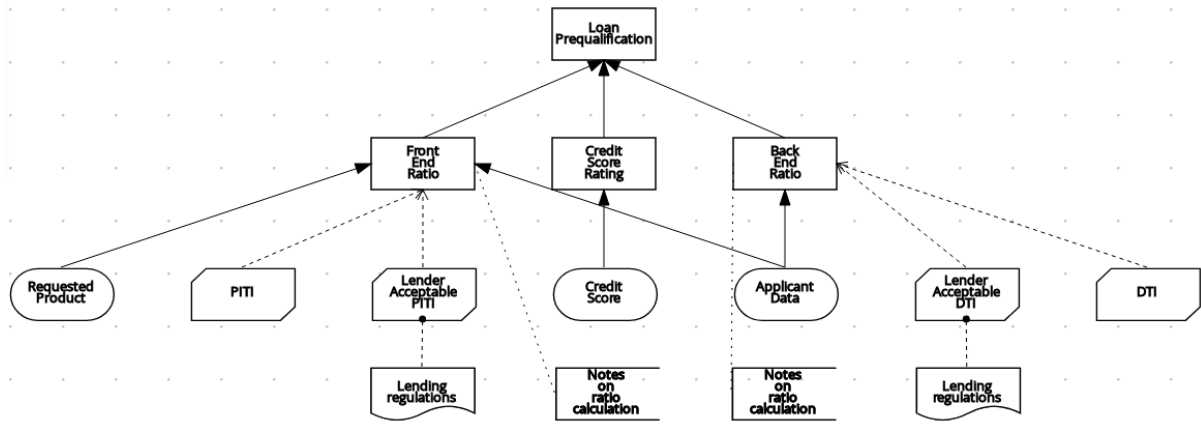
Figure 6.51. Single DRD for loan prequalification
