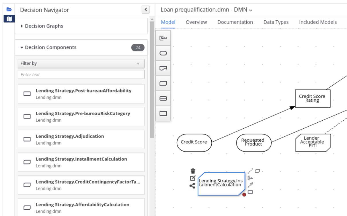
Figure 6.42. Adding DRD components from the included DMN model
