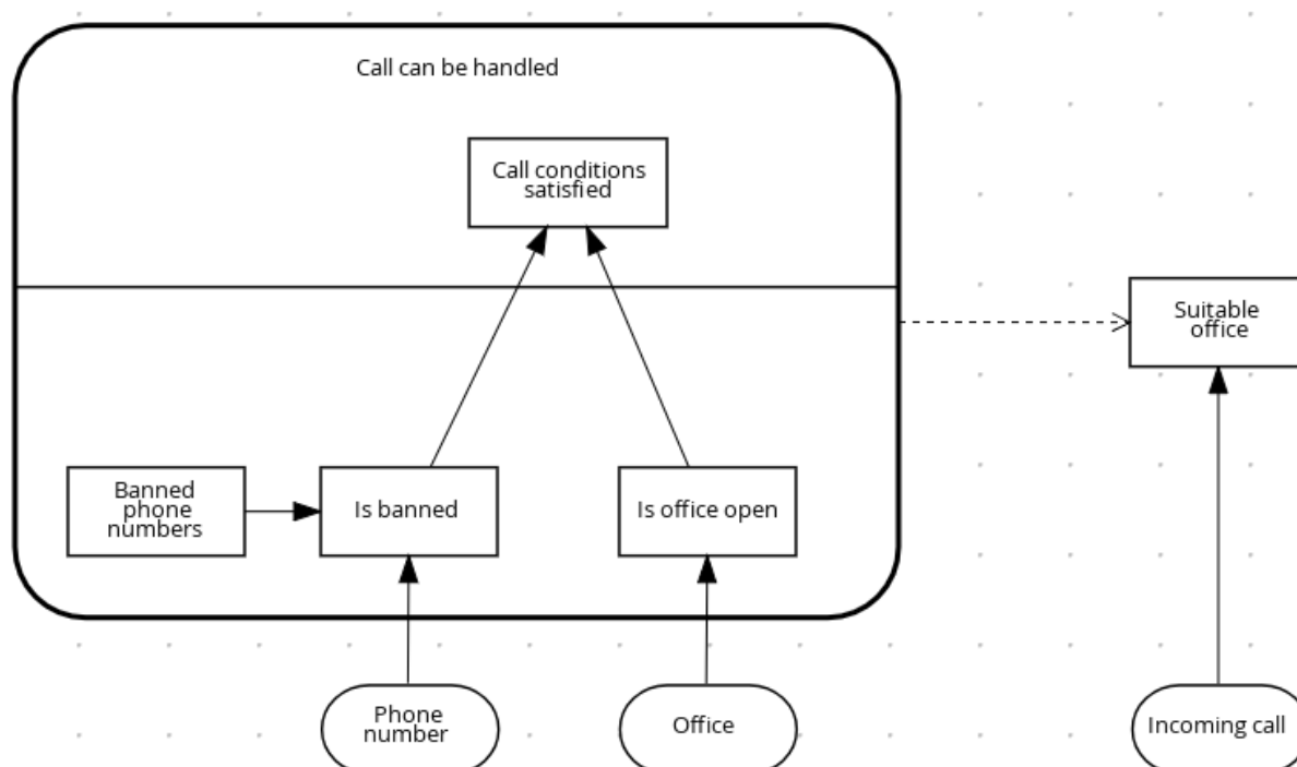
Figure 6.10. Completed DRD for phone call handling with a decision service
