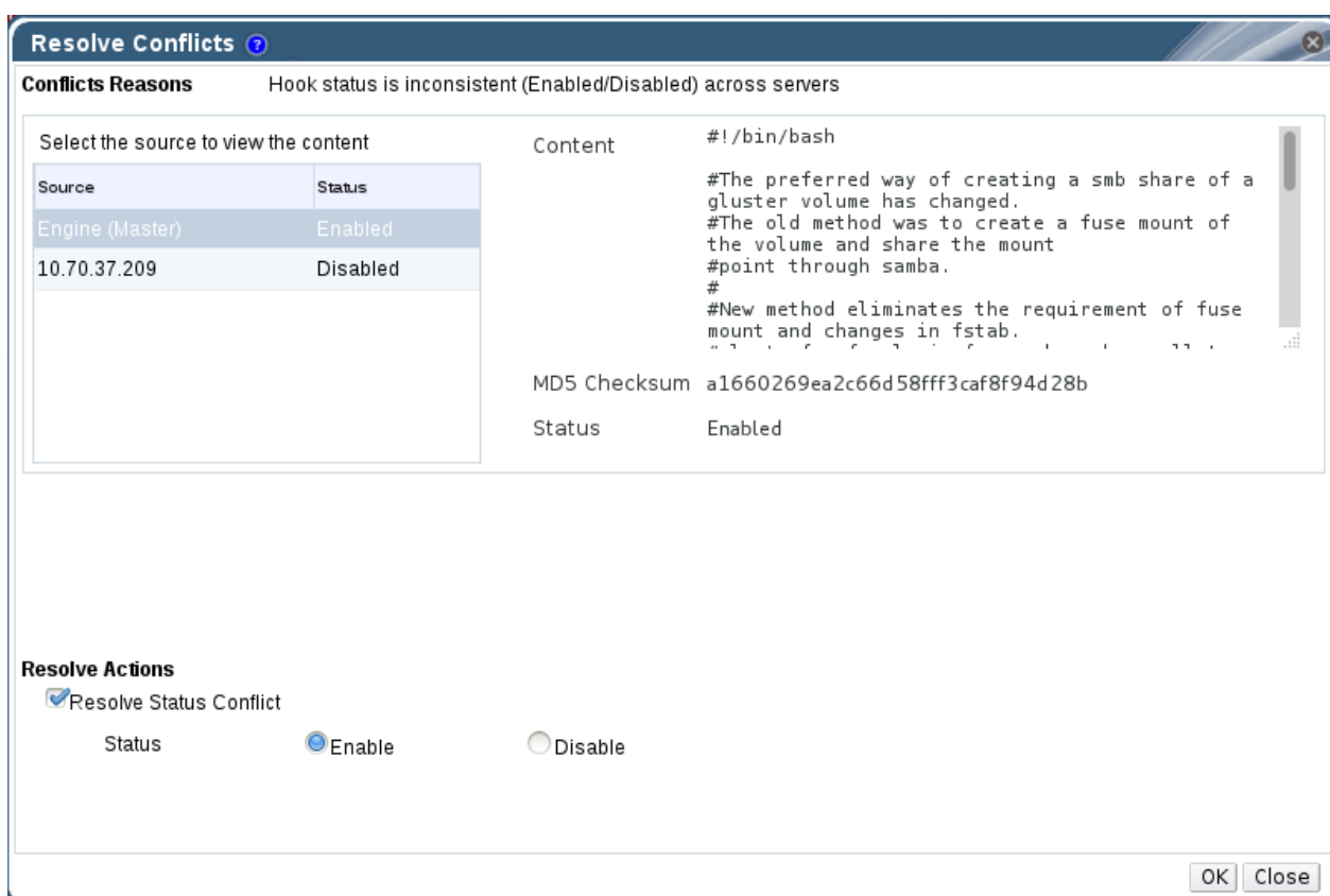
Figure 8.5. Status Conflict
