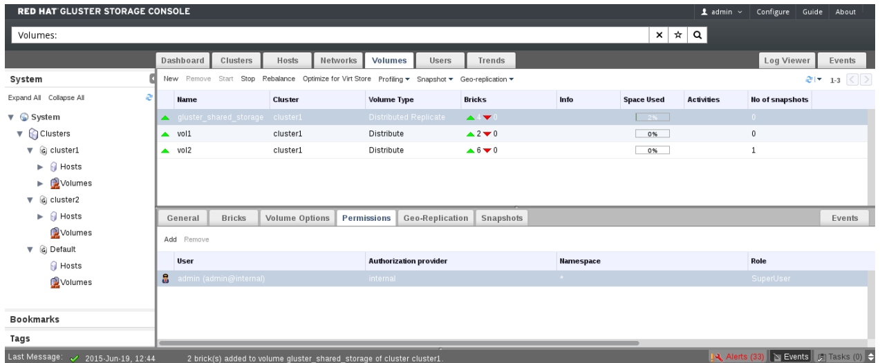
Figure 7.7. Volume Permissions
