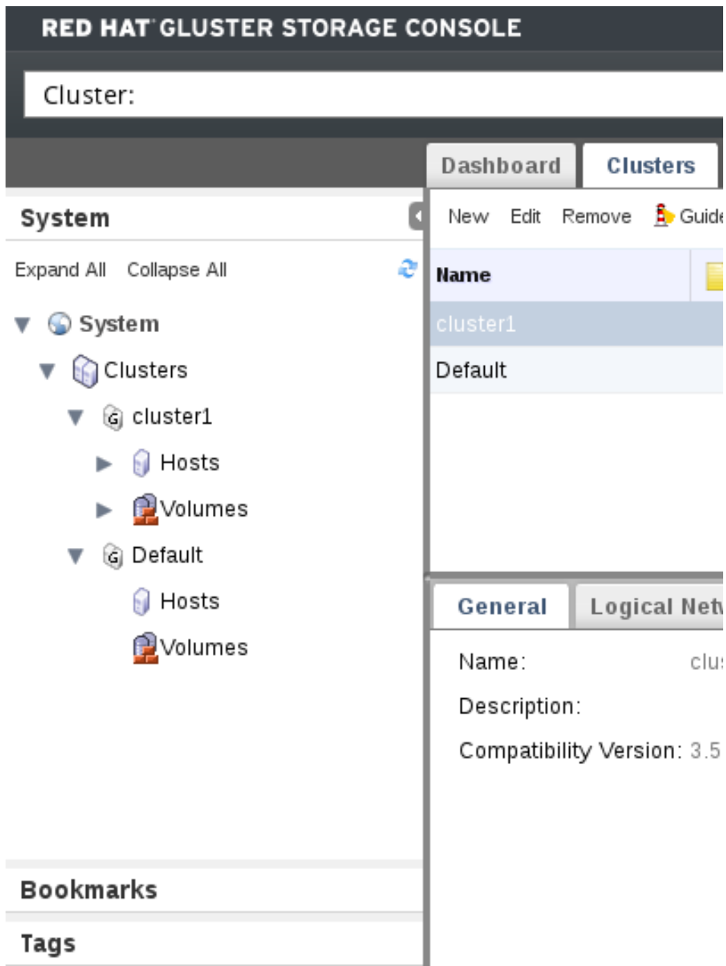
Figure 2.2. Tree Mode
