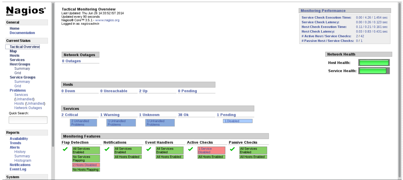
Figure 13.4. Tactical Overview
