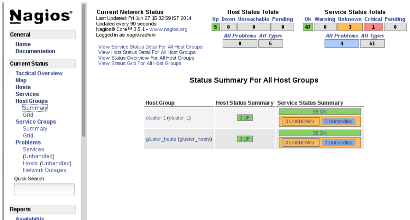
Figure 13.5. Host Groups Summary
