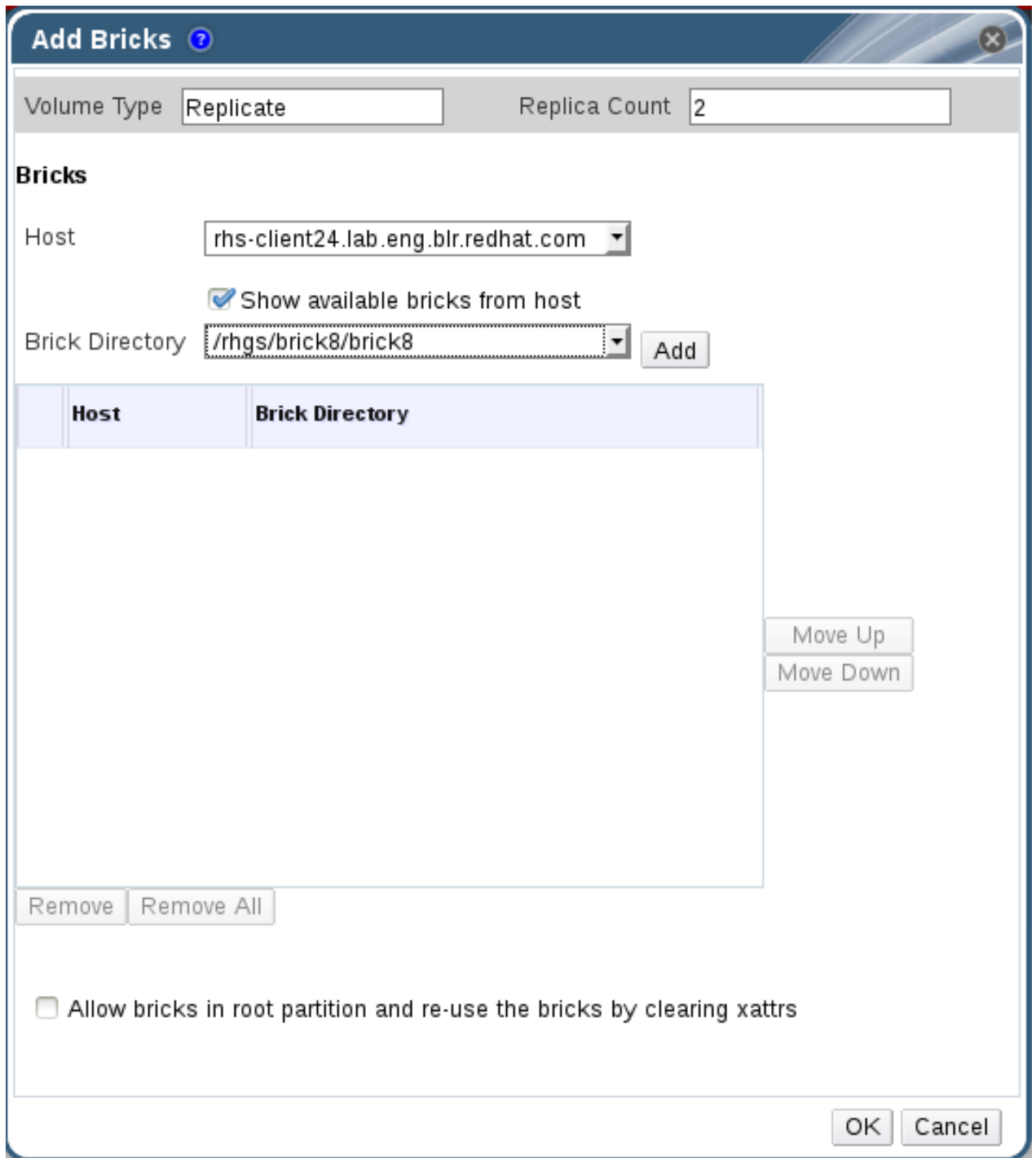
Figure 7.3. Add Bricks
