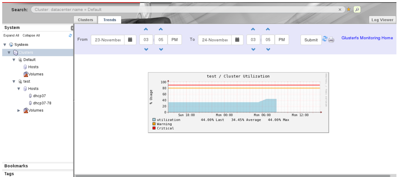
Figure 13.13. Trends
