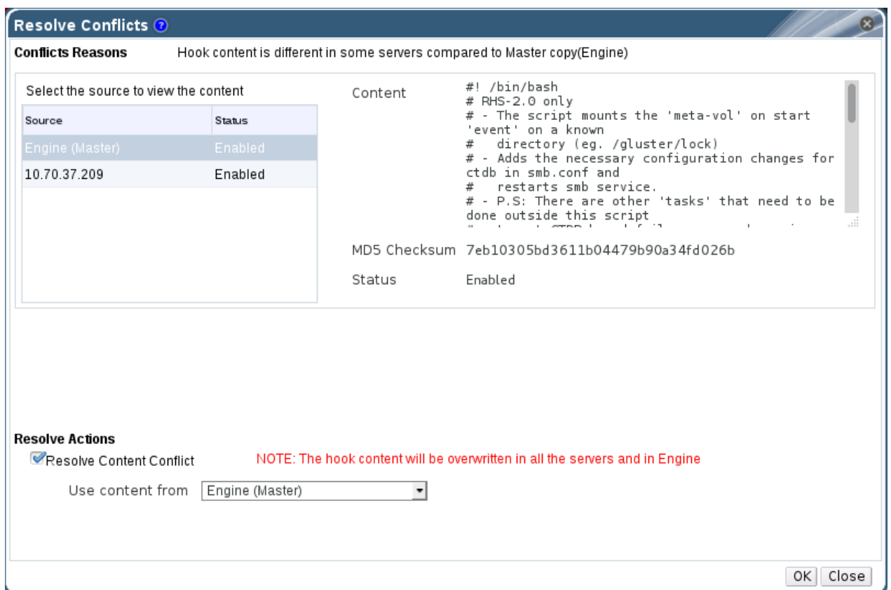
Figure 8.4. Content Conflict
