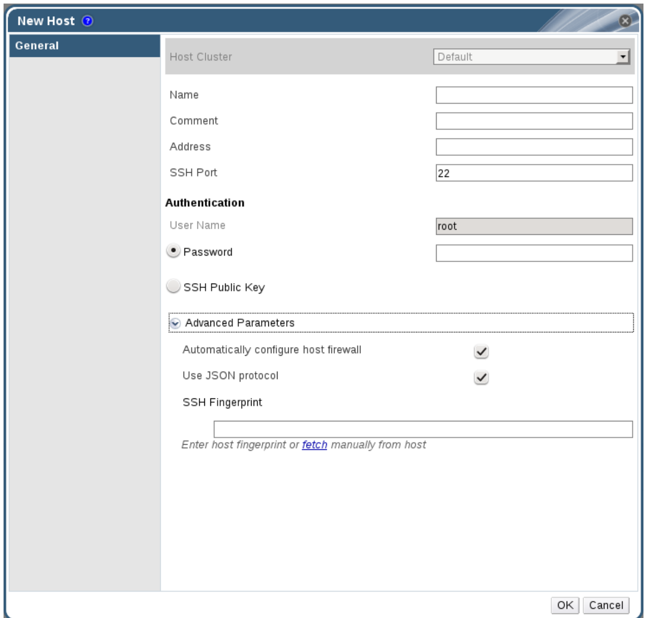
Figure 6.2. New Host Window
